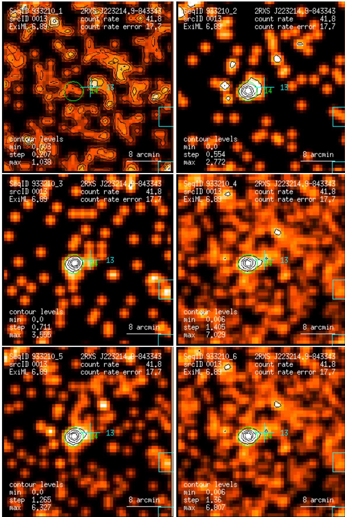
Figure 13: RASS 933210: detection 0013: band rate images, Gaussian filter: (1) PSPC channels 11 – 41, (2) 52 – 90, (3) 91 – 201, (4) 11 – 235, (5) 52 – 201, (6) 11 – 201. Broad band rates in counts/ks. Band rate contour levels in counts/ks/arcmin 2 .
