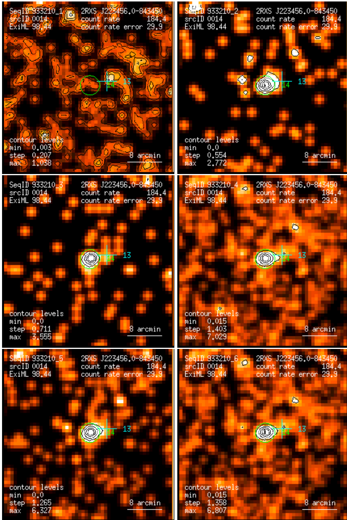
Figure 14: RASS 933210: detection 0014: band rate images, Gaussian filter: (1) PSPC channels 11 – 41, (2) 52 – 90, (3) 91 – 201, (4) 11 – 235, (5) 52 – 201, (6) 11 – 201. Broad band rates in counts/ks. Band rate contour levels in counts/ks/arcmin 2 .
