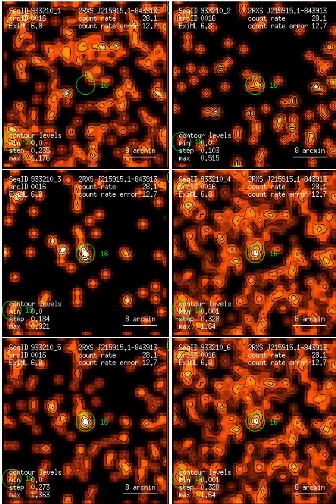
Figure 16: RASS 933210: detection 0016: band rate images, Gaussian filter: (1) PSPC channels 11 – 41, (2) 52 – 90, (3) 91 – 201, (4) 11 – 235, (5) 52 – 201, (6) 11 – 201. Broad band rates in counts/ks. Band rate contour levels in counts/ks/arcmin 2 .
