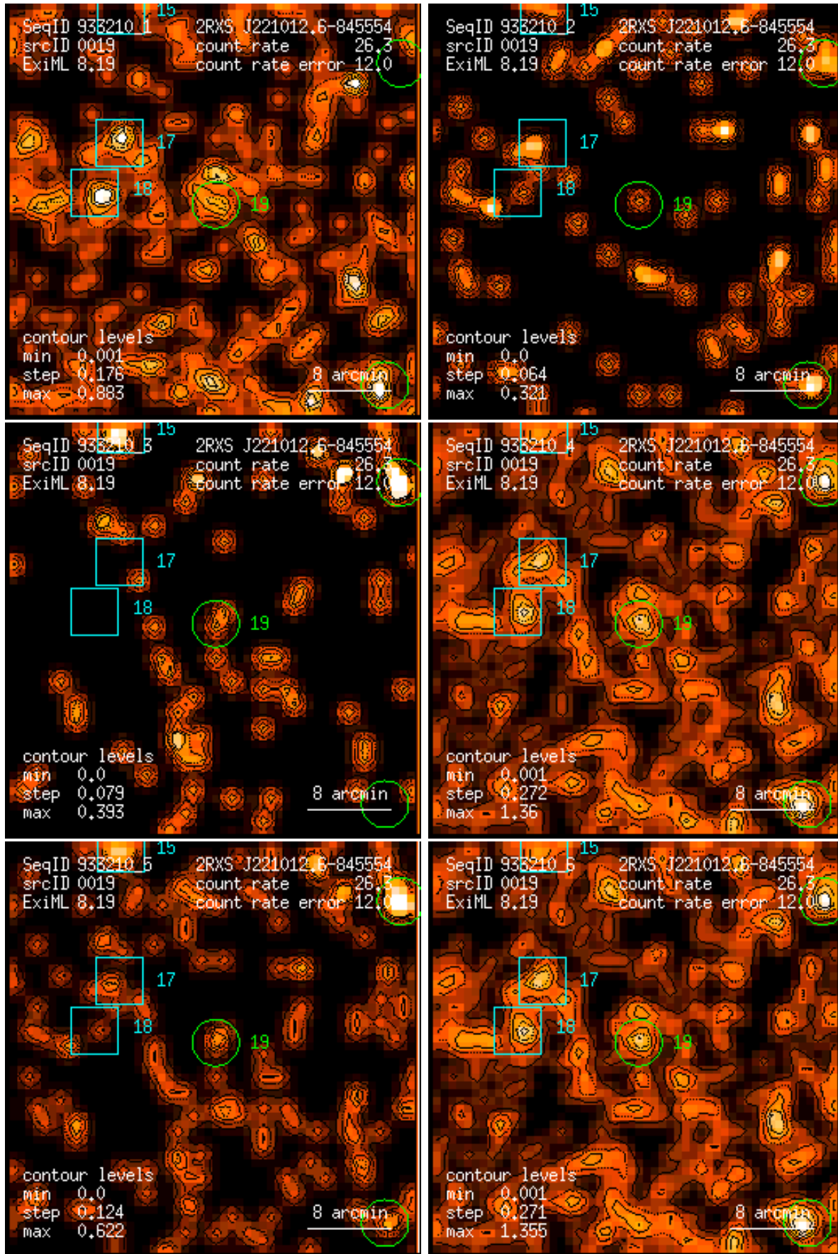
Figure 19: RASS 933210: detection 0019: band rate images, Gaussian filter: (1) PSPC channels 11 – 41, (2) 52 – 90, (3) 91 – 201, (4) 11 – 235, (5) 52 – 201, (6) 11 – 201. Broad band rates in counts/ks. Band rate contour levels in counts/ks/arcmin 2 .
