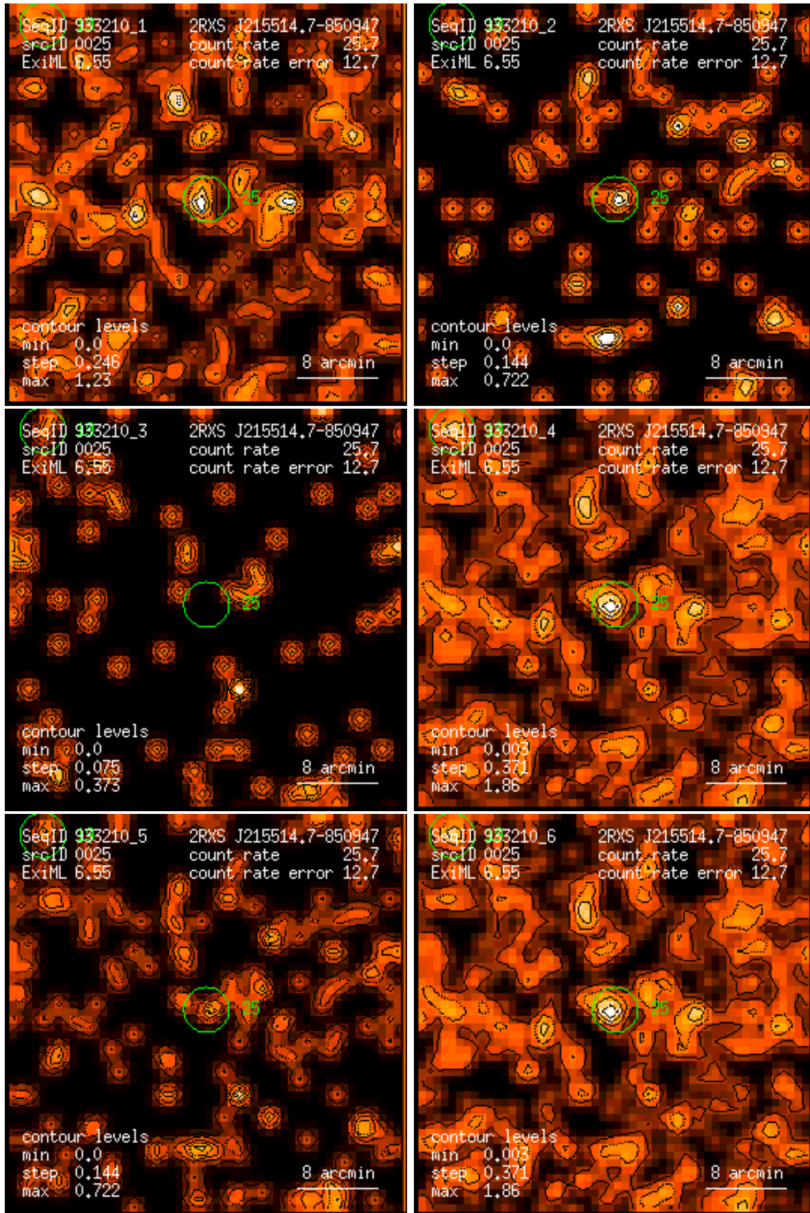
Figure 25: RASS 933210: detection 0025: band rate images, Gaussian filter: (1) PSPC channels 11 – 41, (2) 52 – 90, (3) 91 – 201, (4) 11 – 235, (5) 52 – 201, (6) 11 – 201. Broad band rates in counts/ks. Band rate contour levels in counts/ks/arcmin 2 .
