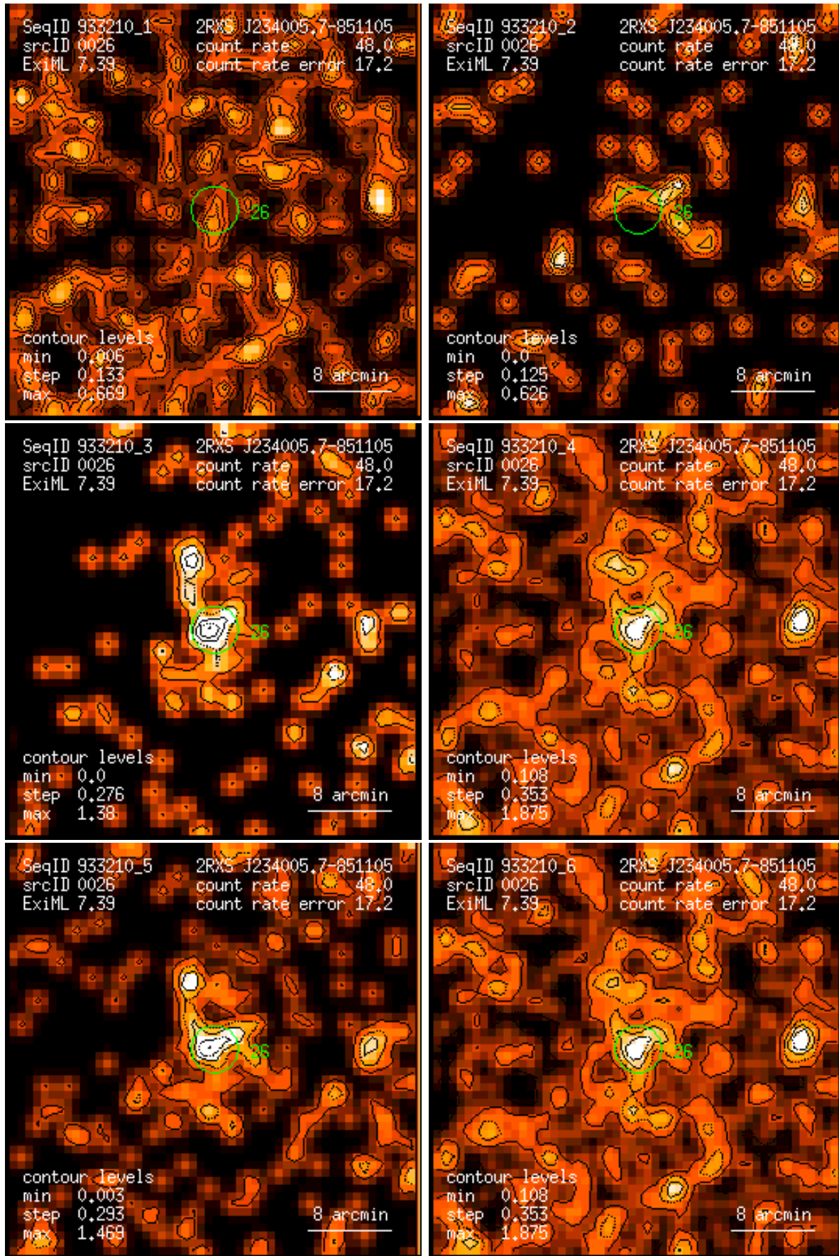
Figure 26: RASS 933210: detection 0026: band rate images, Gaussian filter: (1) PSPC channels 11 – 41, (2) 52 – 90, (3) 91 – 201, (4) 11 – 235, (5) 52 – 201, (6) 11 – 201. Broad band rates in counts/ks. Band rate contour levels in counts/ks/arcmin 2 .
