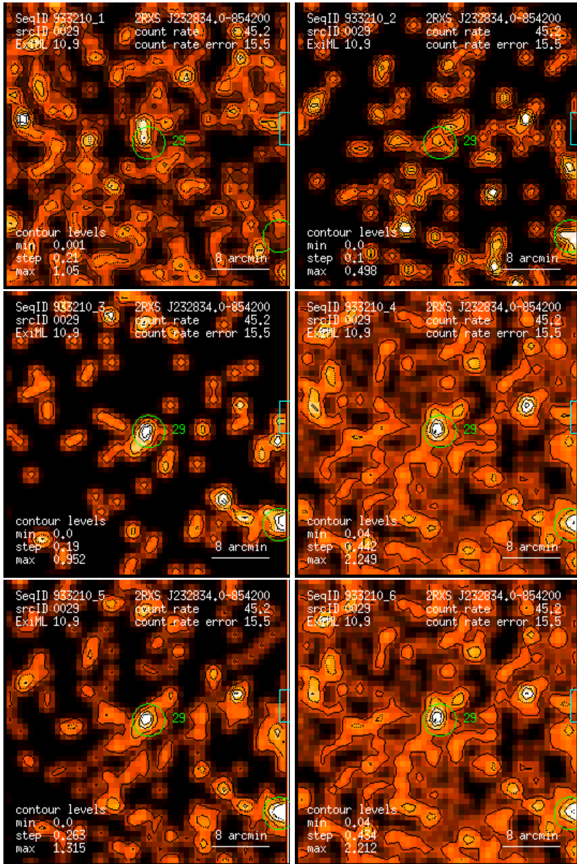
Figure 29: RASS 933210: detection 0029: band rate images, Gaussian filter: (1) PSPC channels 11 – 41, (2) 52 – 90, (3) 91 – 201, (4) 11 – 235, (5) 52 – 201, (6) 11 – 201. Broad band rates in counts/ks. Band rate contour levels in counts/ks/arcmin 2 .
