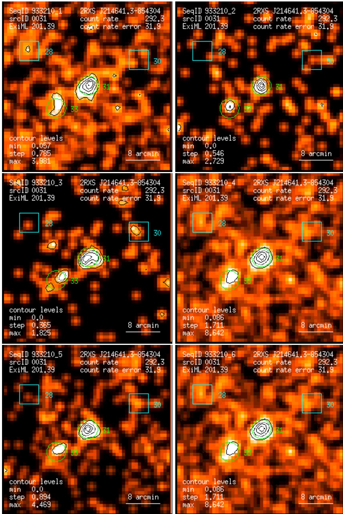
Figure 31: RASS 933210: detection 0031: band rate images, Gaussian filter: (1) PSPC channels 11 – 41, (2) 52 – 90, (3) 91 – 201, (4) 11 – 235, (5) 52 – 201, (6) 11 – 201. Broad band rates in counts/ks. Band rate contour levels in counts/ks/arcmin 2 .
