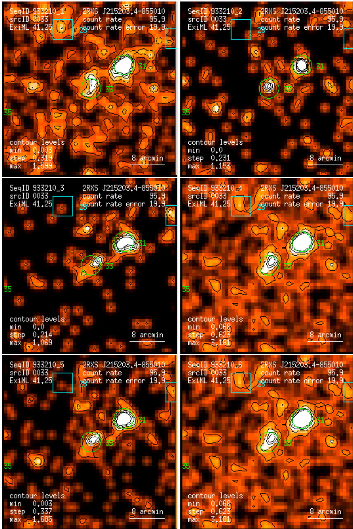
Figure 33: RASS 933210: detection 0033: band rate images, Gaussian filter: (1) PSPC channels 11 – 41, (2) 52 – 90, (3) 91 – 201, (4) 11 – 235, (5) 52 – 201, (6) 11 – 201. Broad band rates in counts/ks. Band rate contour levels in counts/ks/arcmin 2 .
