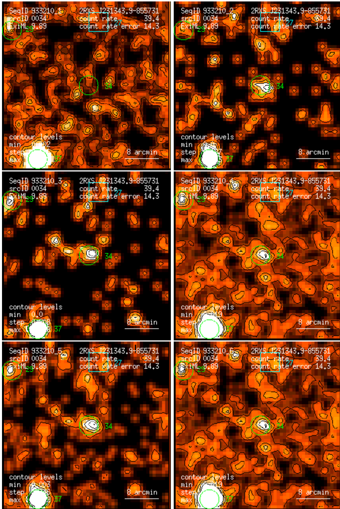
Figure 34: RASS 933210: detection 0034: band rate images, Gaussian filter: (1) PSPC channels 11 – 41, (2) 52 – 90, (3) 91 – 201, (4) 11 – 235, (5) 52 – 201, (6) 11 – 201. Broad band rates in counts/ks. Band rate contour levels in counts/ks/arcmin 2 .
