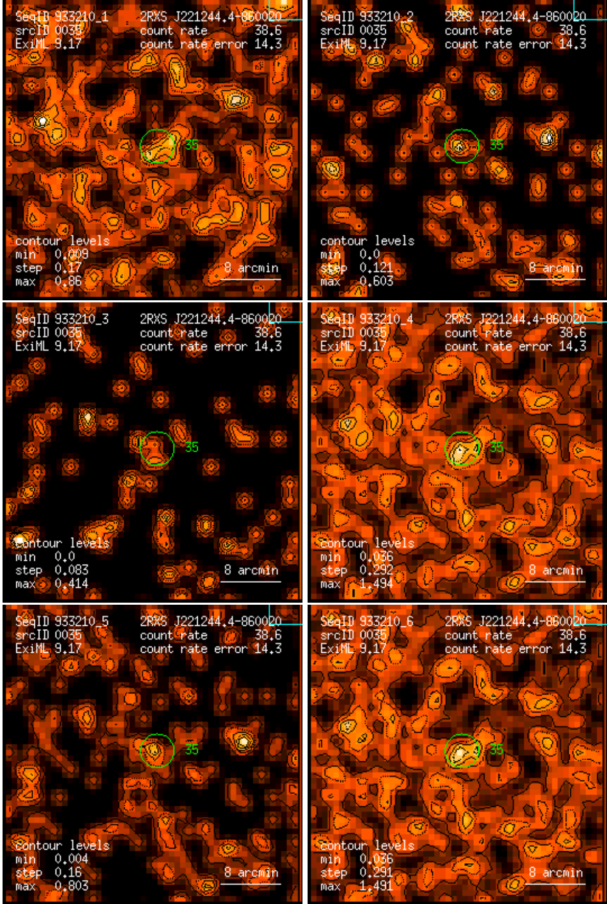
Figure 35: RASS 933210: detection 0035: band rate images, Gaussian filter: (1) PSPC channels 11 – 41, (2) 52 – 90, (3) 91 – 201, (4) 11 – 235, (5) 52 – 201, (6) 11 – 201. Broad band rates in counts/ks. Band rate contour levels in counts/ks/arcmin 2 .
