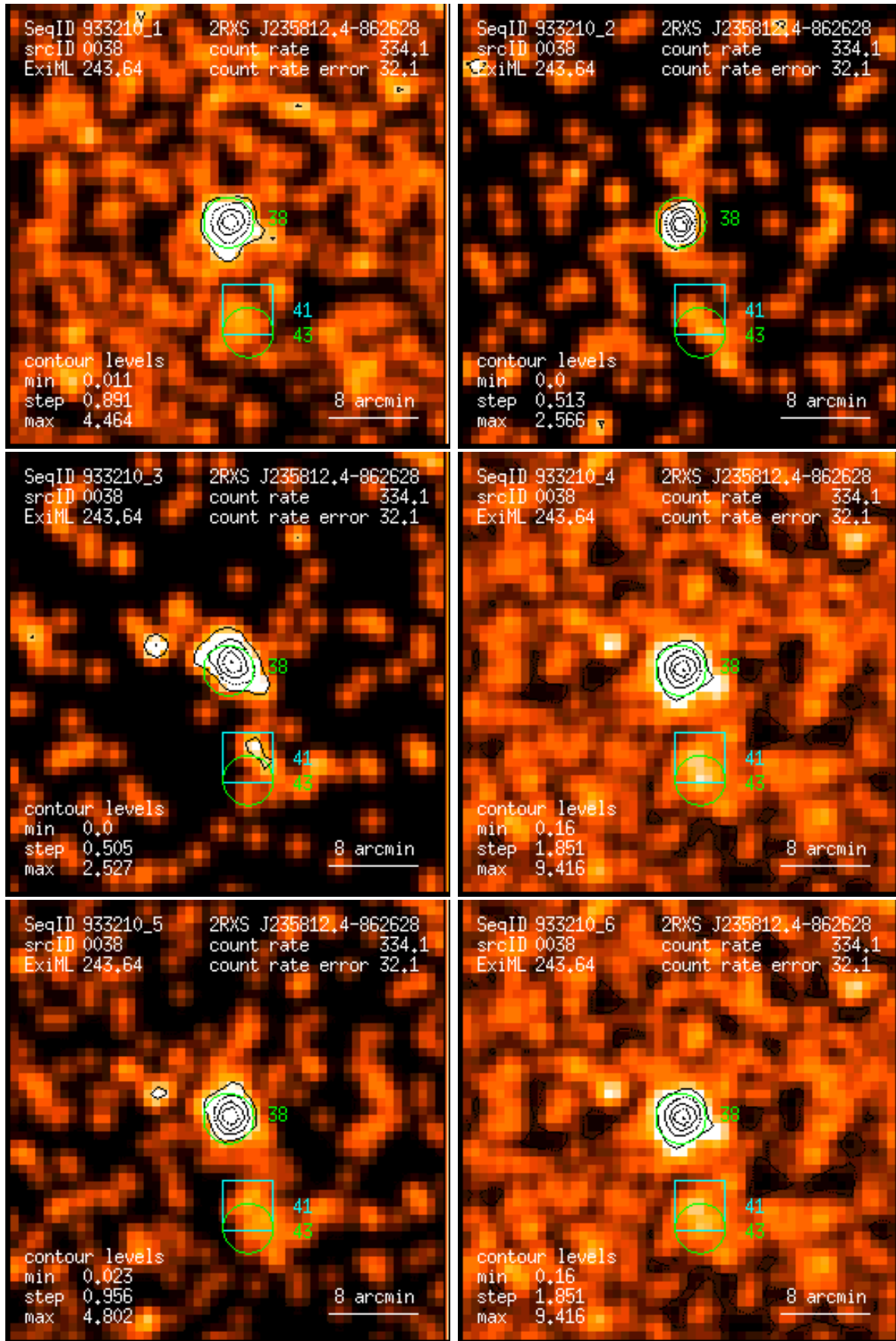
Figure 38: RASS 933210: detection 0038: band rate images, Gaussian filter: (1) PSPC channels 11 – 41, (2) 52 – 90, (3) 91 – 201, (4) 11 – 235, (5) 52 – 201, (6) 11 – 201. Broad band rates in counts/ks. Band rate contour levels in counts/ks/arcmin 2 .
