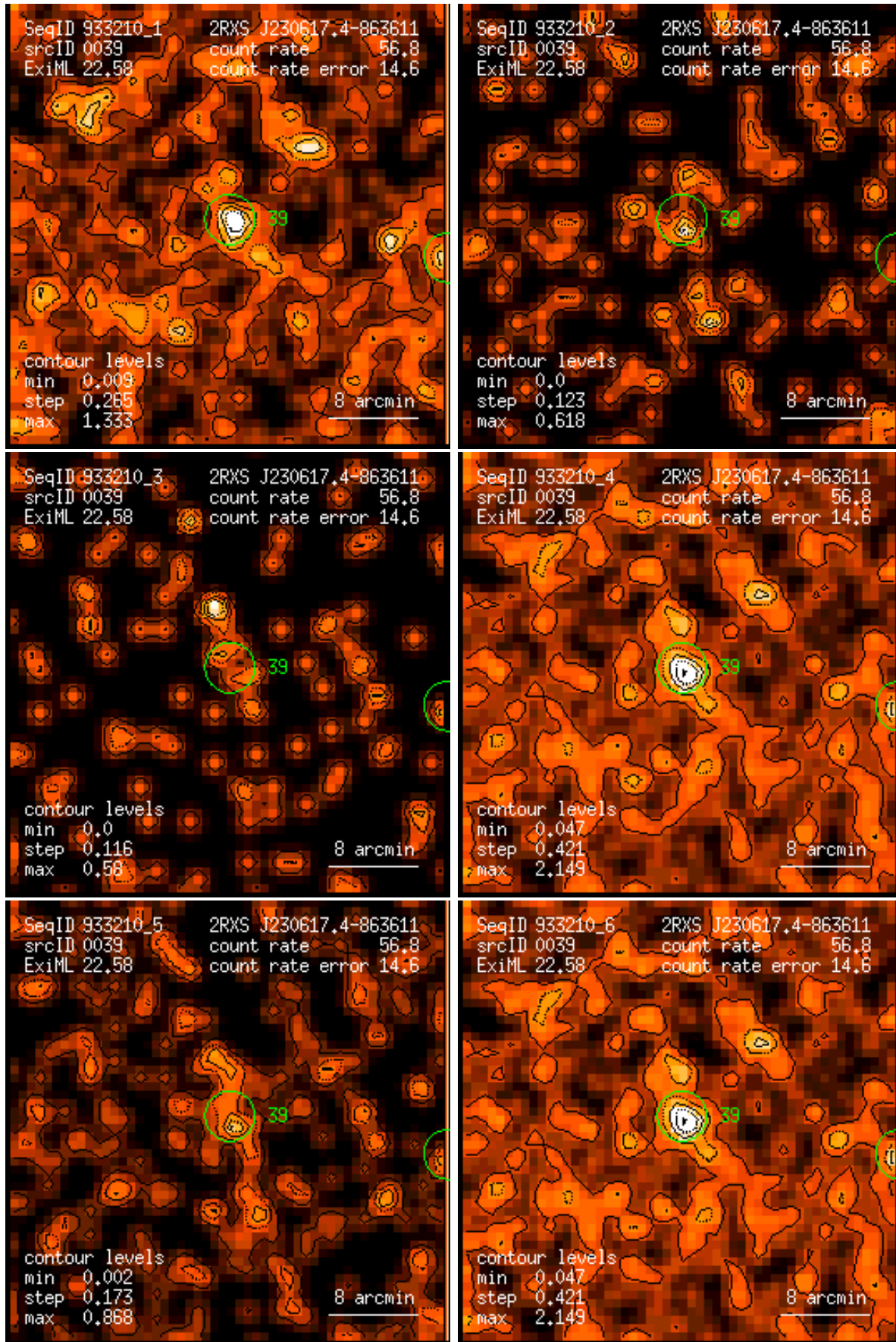
Figure 39: RASS 933210: detection 0039: band rate images, Gaussian filter: (1) PSPC channels 11 – 41, (2) 52 – 90, (3) 91 – 201, (4) 11 – 235, (5) 52 – 201, (6) 11 – 201. Broad band rates in counts/ks. Band rate contour levels in counts/ks/arcmin 2 .
