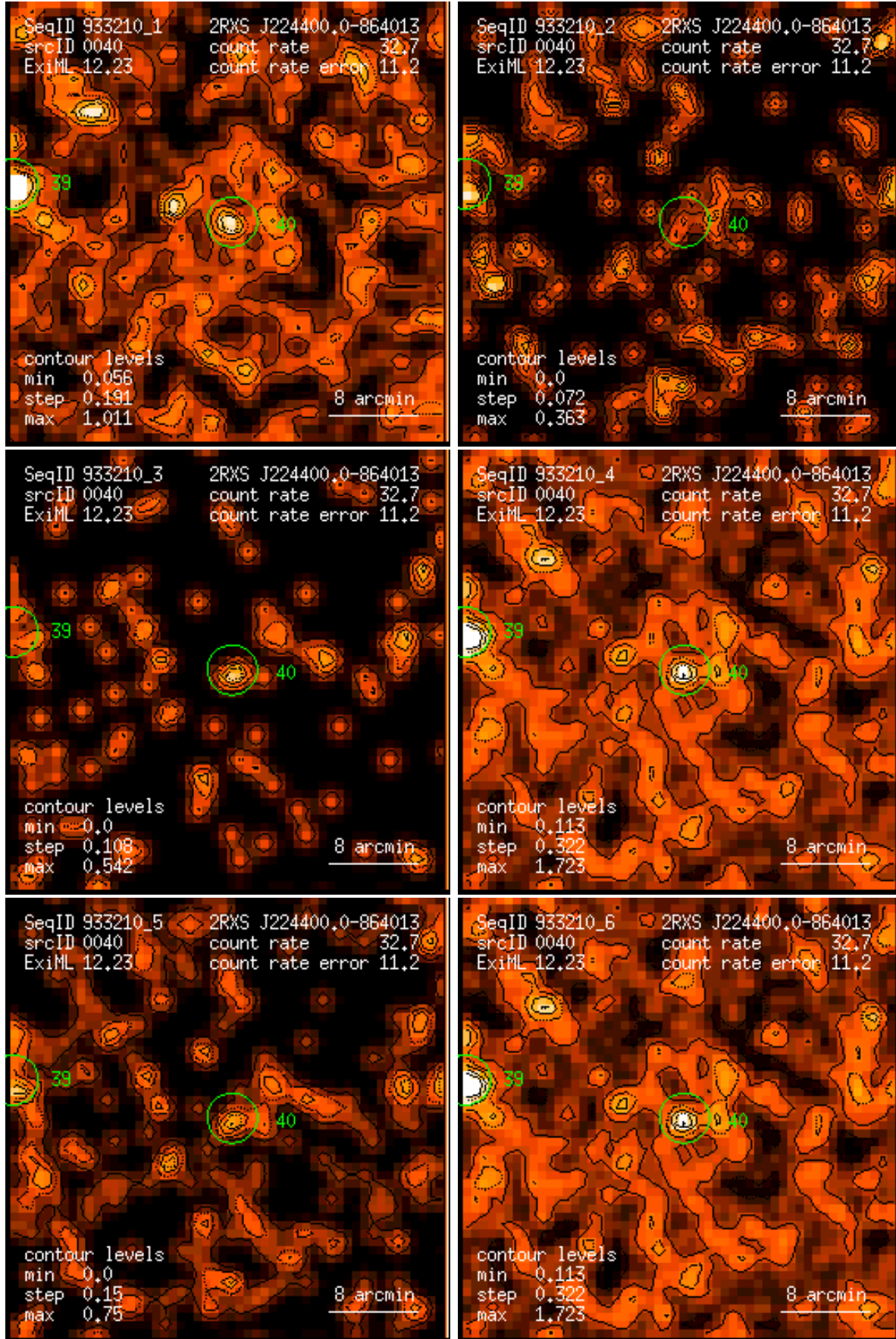
Figure 40: RASS 933210: detection 0040: band rate images, Gaussian filter: (1) PSPC channels 11 – 41, (2) 52 – 90, (3) 91 – 201, (4) 11 – 235, (5) 52 – 201, (6) 11 – 201. Broad band rates in counts/ks. Band rate contour levels in counts/ks/arcmin 2 .
