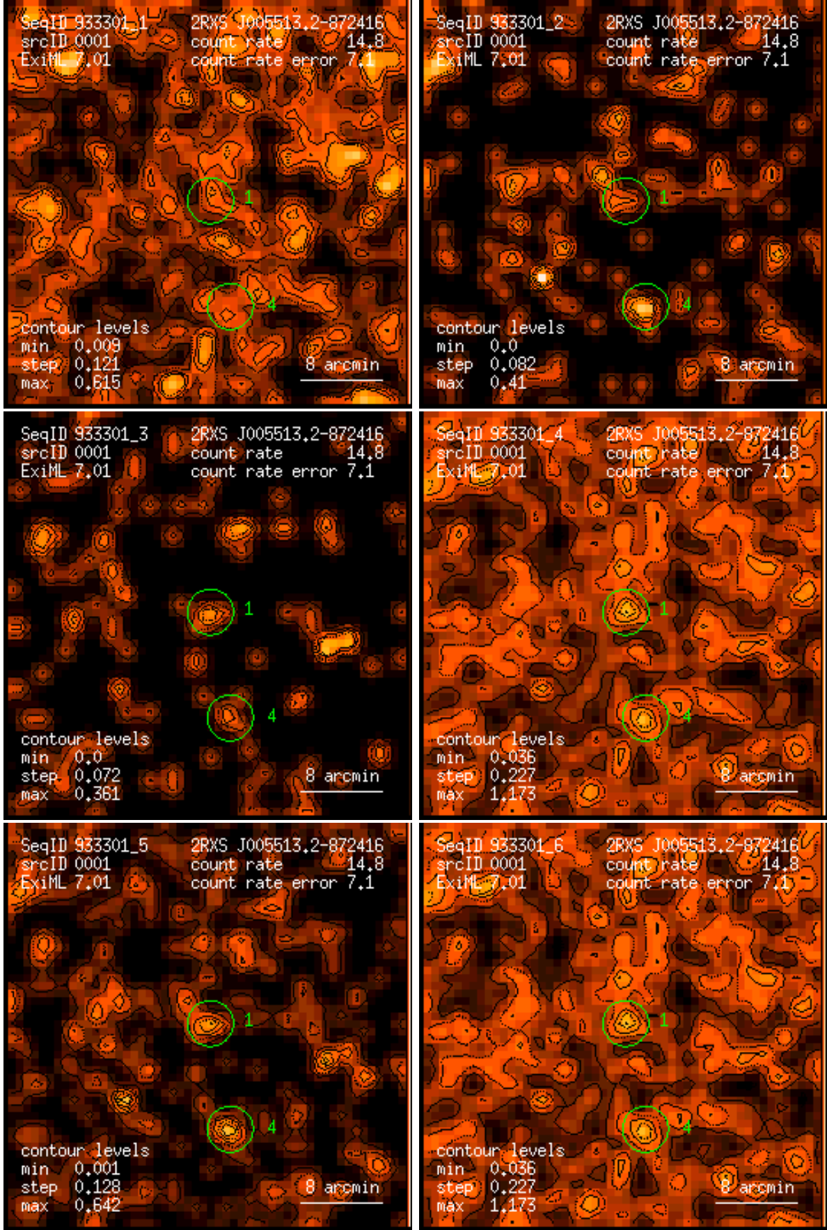
Figure 1: RASS 933301: detection 0001: band rate images, Gaussian filter: (1) PSPC channels 11 – 41, (2) 52 – 90, (3) 91 – 201, (4) 11 – 235, (5) 52 – 201, (6) 11 – 201. Broad band rates in counts/ks. Band rate contour levels in counts/ks/arcmin 2 .
