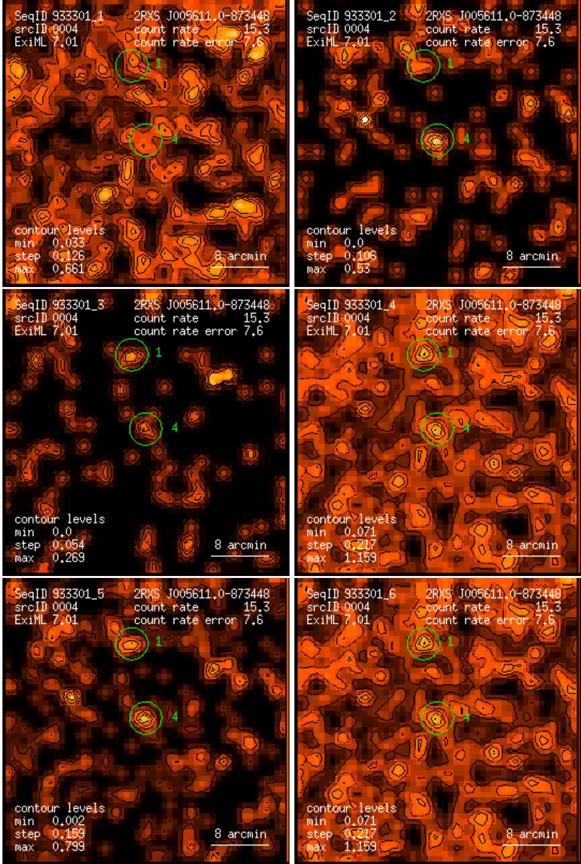
Figure 4: RASS 933301: detection 0004: band rate images, Gaussian filter: (1) PSPC channels 11 – 41, (2) 52 – 90, (3) 91 – 201, (4) 11 – 235, (5) 52 – 201, (6) 11 – 201. Broad band rates in counts/ks. Band rate contour levels in counts/ks/arcmin 2 .
