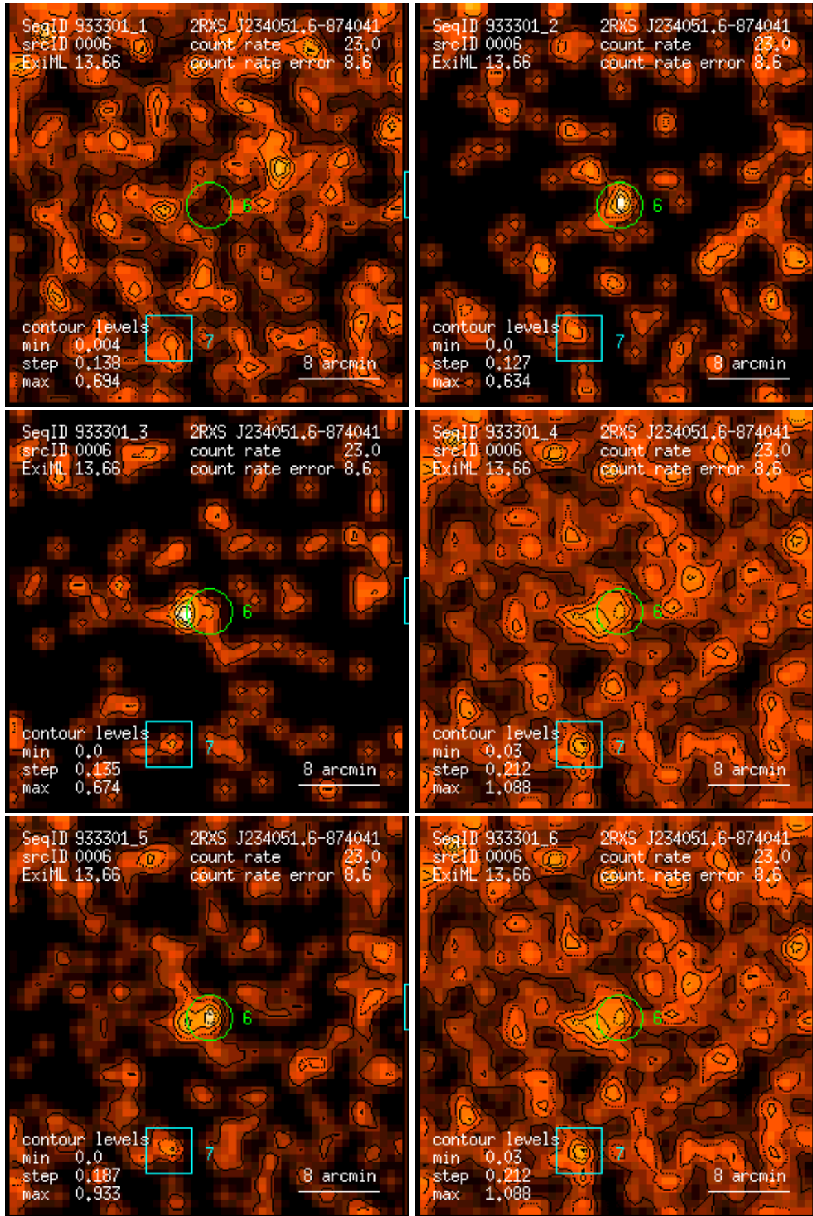
Figure 6: RASS 933301: detection 0006: band rate images, Gaussian filter: (1) PSPC channels 11 – 41, (2) 52 – 90, (3) 91 – 201, (4) 11 – 235, (5) 52 – 201, (6) 11 – 201. Broad band rates in counts/ks. Band rate contour levels in counts/ks/arcmin 2 .
