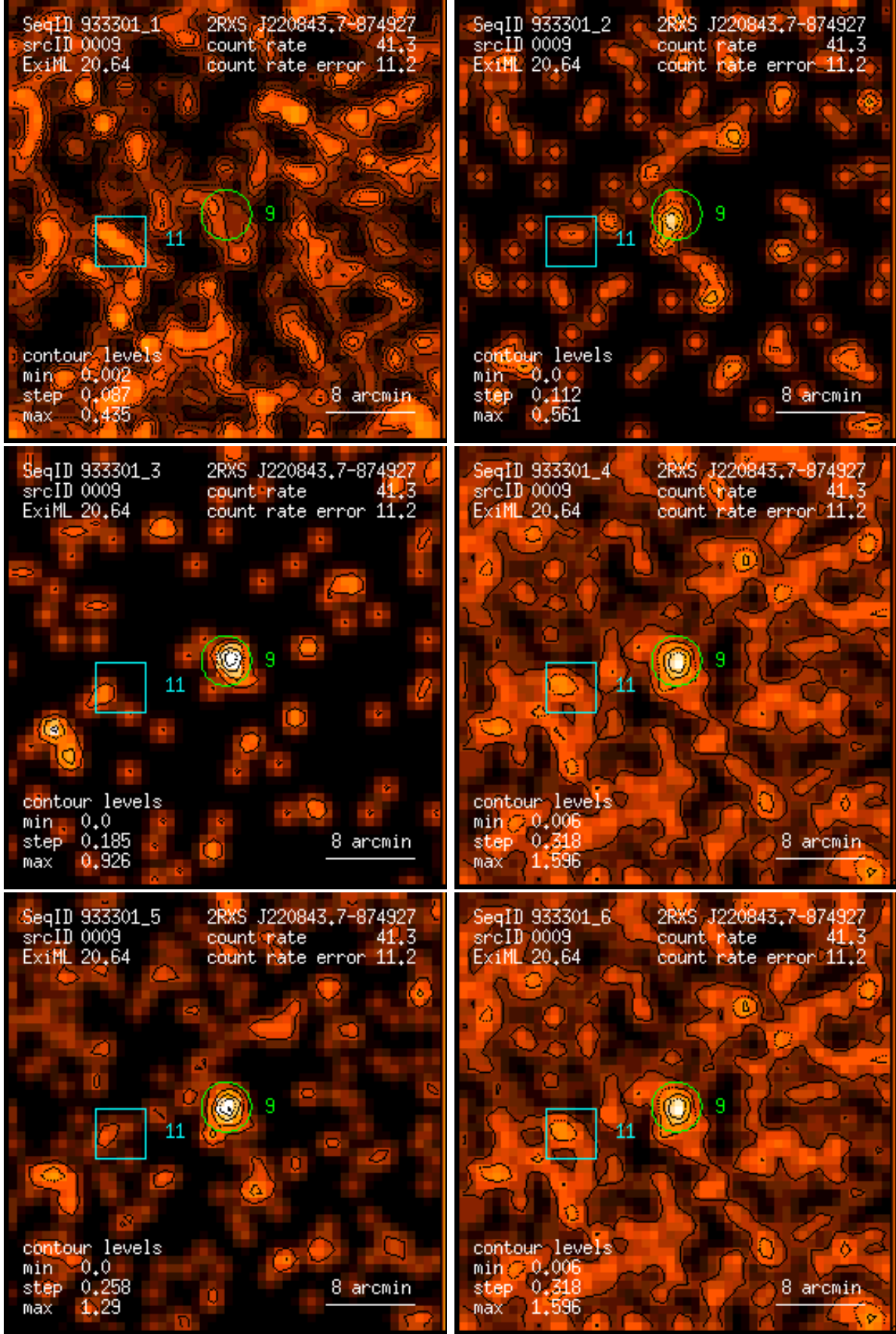
Figure 9: RASS 933301: detection 0009: band rate images, Gaussian filter: (1) PSPC channels 11 – 41, (2) 52 – 90, (3) 91 – 201, (4) 11 – 235, (5) 52 – 201, (6) 11 – 201. Broad band rates in counts/ks. Band rate contour levels in counts/ks/arcmin 2 .
