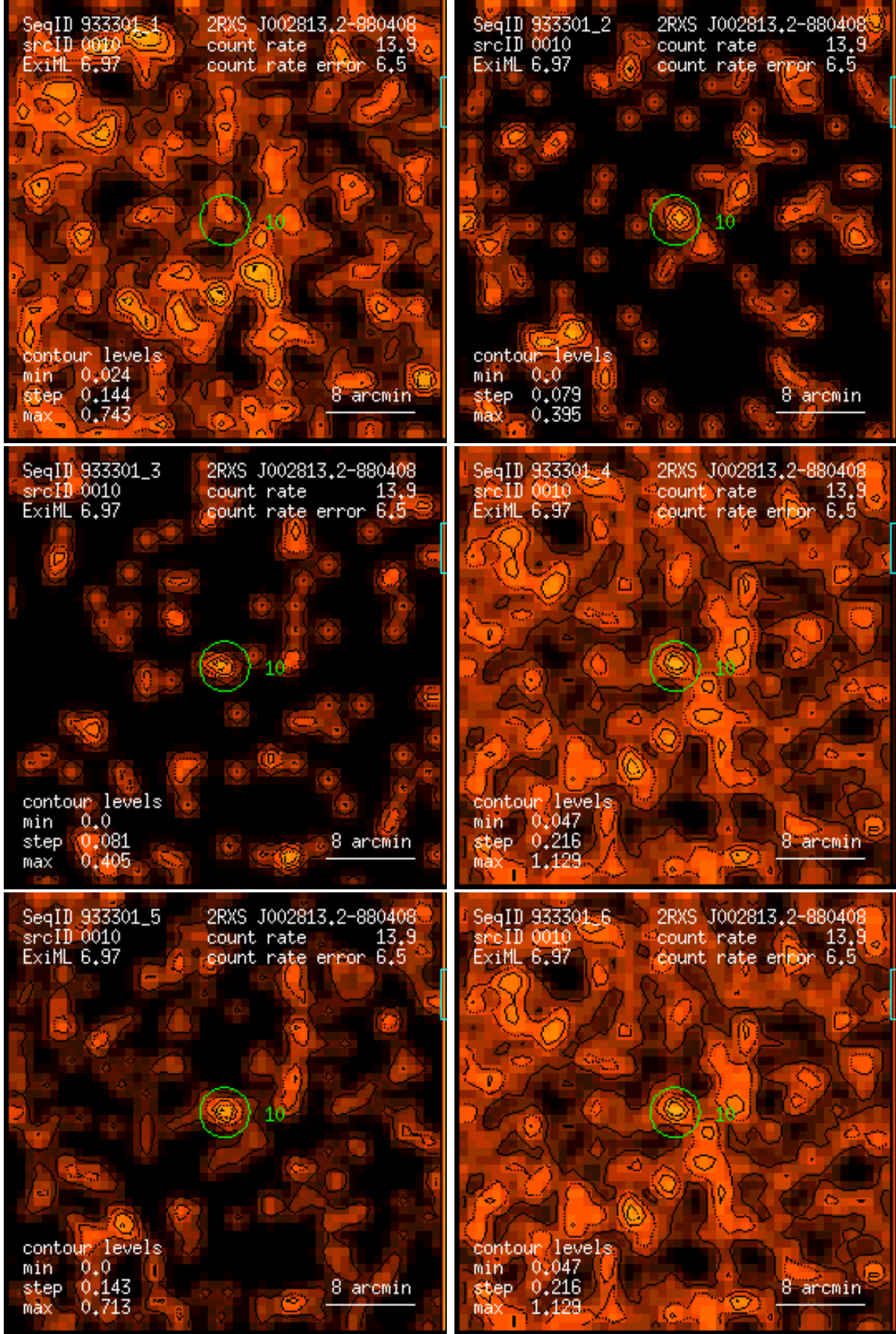
Figure 10: RASS 933301: detection 0010: band rate images, Gaussian filter: (1) PSPC channels 11 – 41, (2) 52 – 90, (3) 91 – 201, (4) 11 – 235, (5) 52 – 201, (6) 11 – 201. Broad band rates in counts/ks. Band rate contour levels in counts/ks/arcmin 2 .
