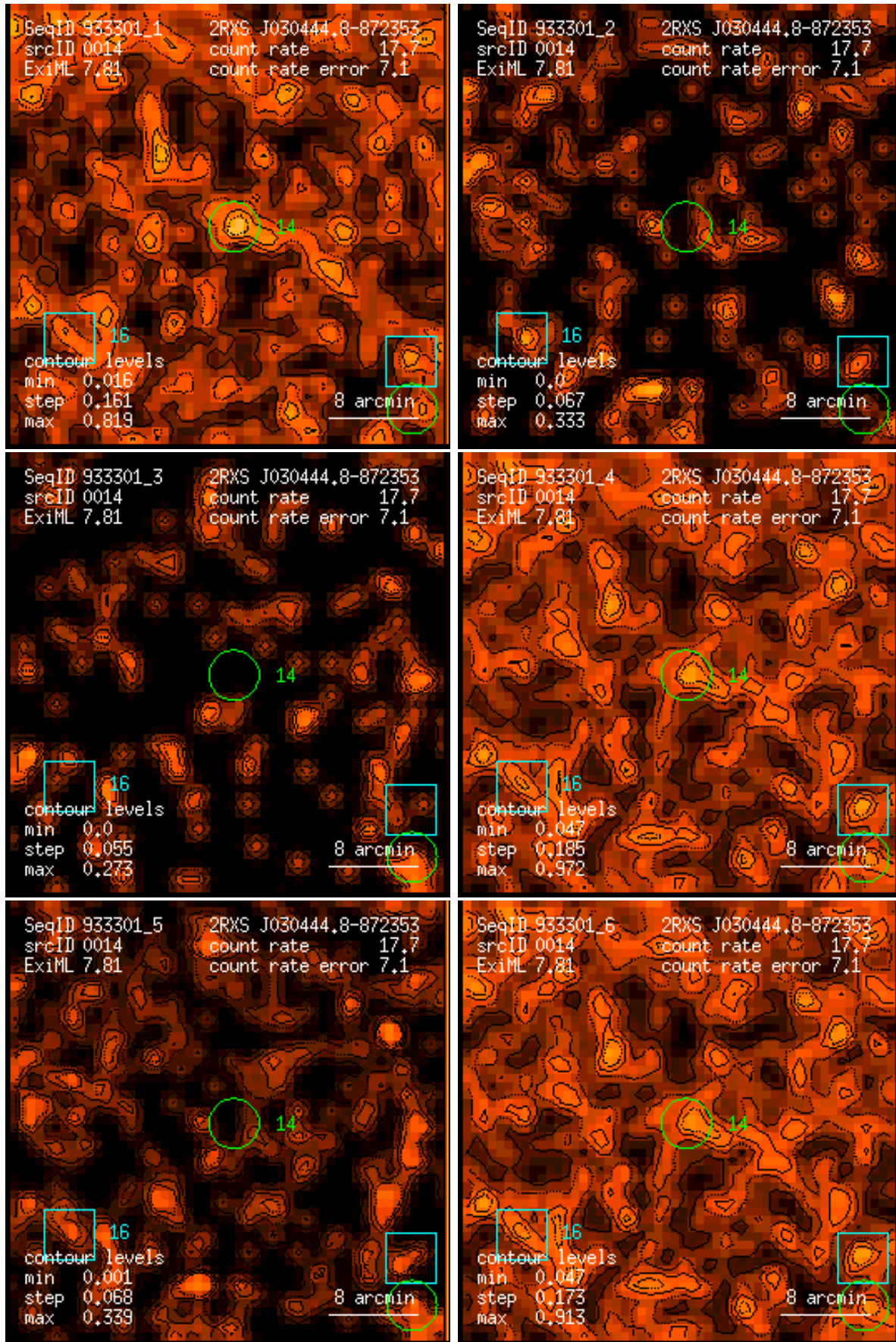
Figure 14: RASS 933301: detection 0014: band rate images, Gaussian filter: (1) PSPC channels 11 – 41, (2) 52 – 90, (3) 91 – 201, (4) 11 – 235, (5) 52 – 201, (6) 11 – 201. Broad band rates in counts/ks. Band rate contour levels in counts/ks/arcmin 2 .
