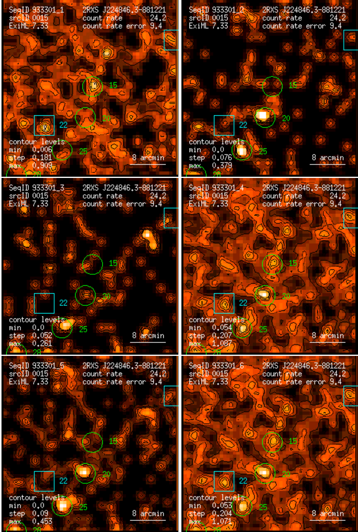
Figure 15: RASS 933301: detection 0015: band rate images, Gaussian filter: (1) PSPC channels 11 – 41, (2) 52 – 90, (3) 91 – 201, (4) 11 – 235, (5) 52 – 201, (6) 11 – 201. Broad band rates in counts/ks. Band rate contour levels in counts/ks/arcmin 2 .
