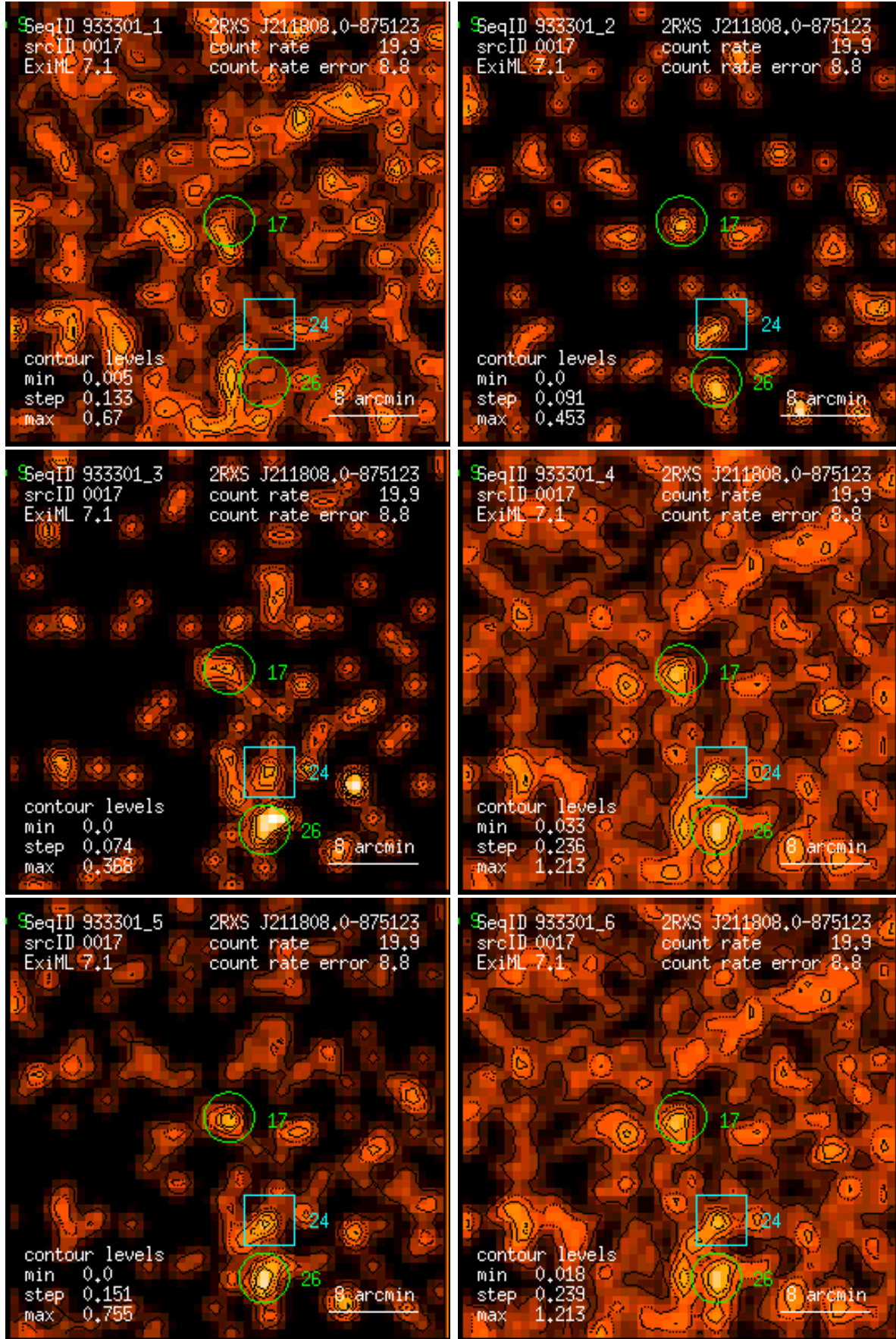
Figure 17: RASS 933301: detection 0017: band rate images, Gaussian filter: (1) PSPC channels 11 – 41, (2) 52 – 90, (3) 91 – 201, (4) 11 – 235, (5) 52 – 201, (6) 11 – 201. Broad band rates in counts/ks. Band rate contour levels in counts/ks/arcmin 2 .
