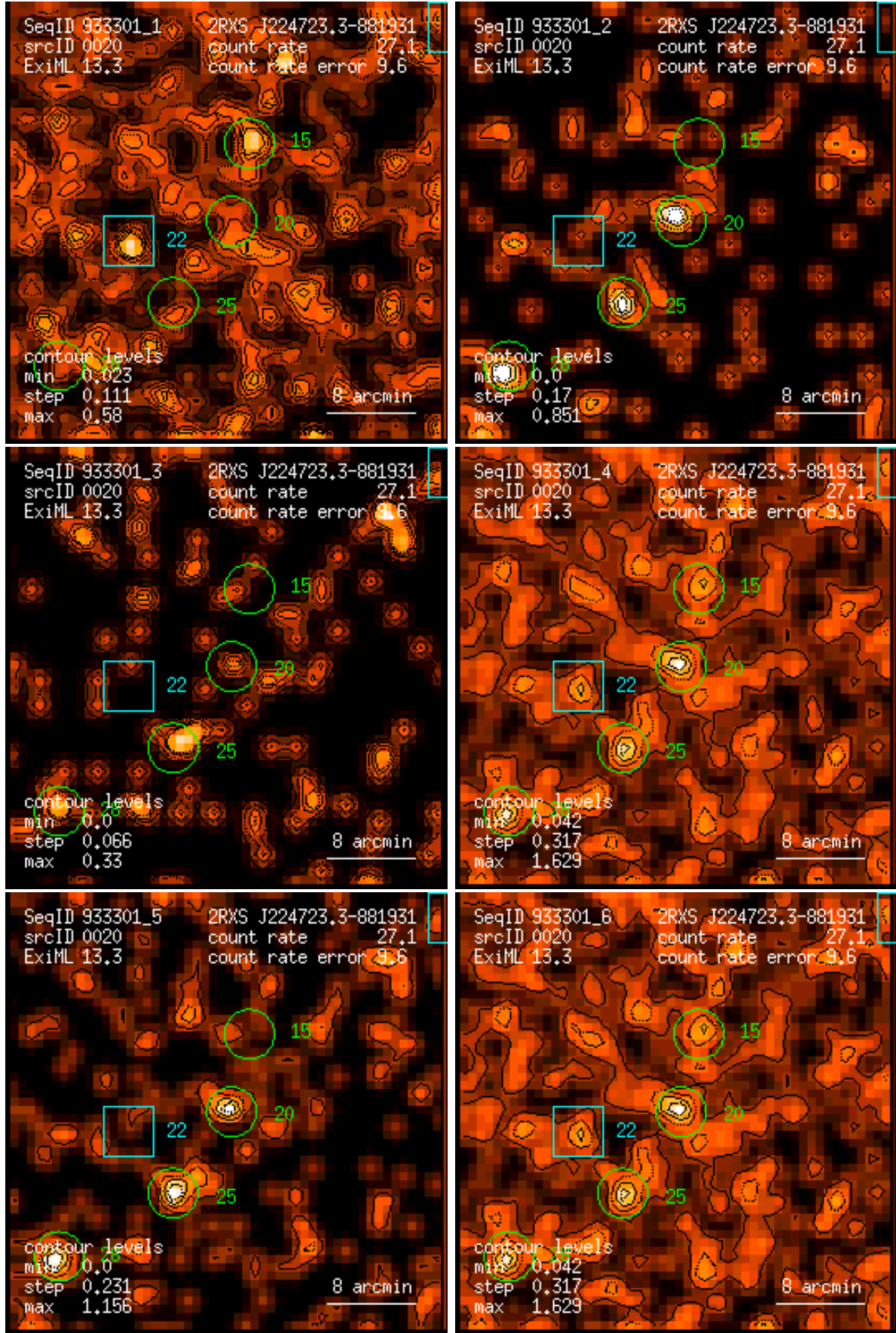
Figure 20: RASS 933301: detection 0020: band rate images, Gaussian filter: (1) PSPC channels 11 – 41, (2) 52 – 90, (3) 91 – 201, (4) 11 – 235, (5) 52 – 201, (6) 11 – 201. Broad band rates in counts/ks. Band rate contour levels in counts/ks/arcmin 2 .
