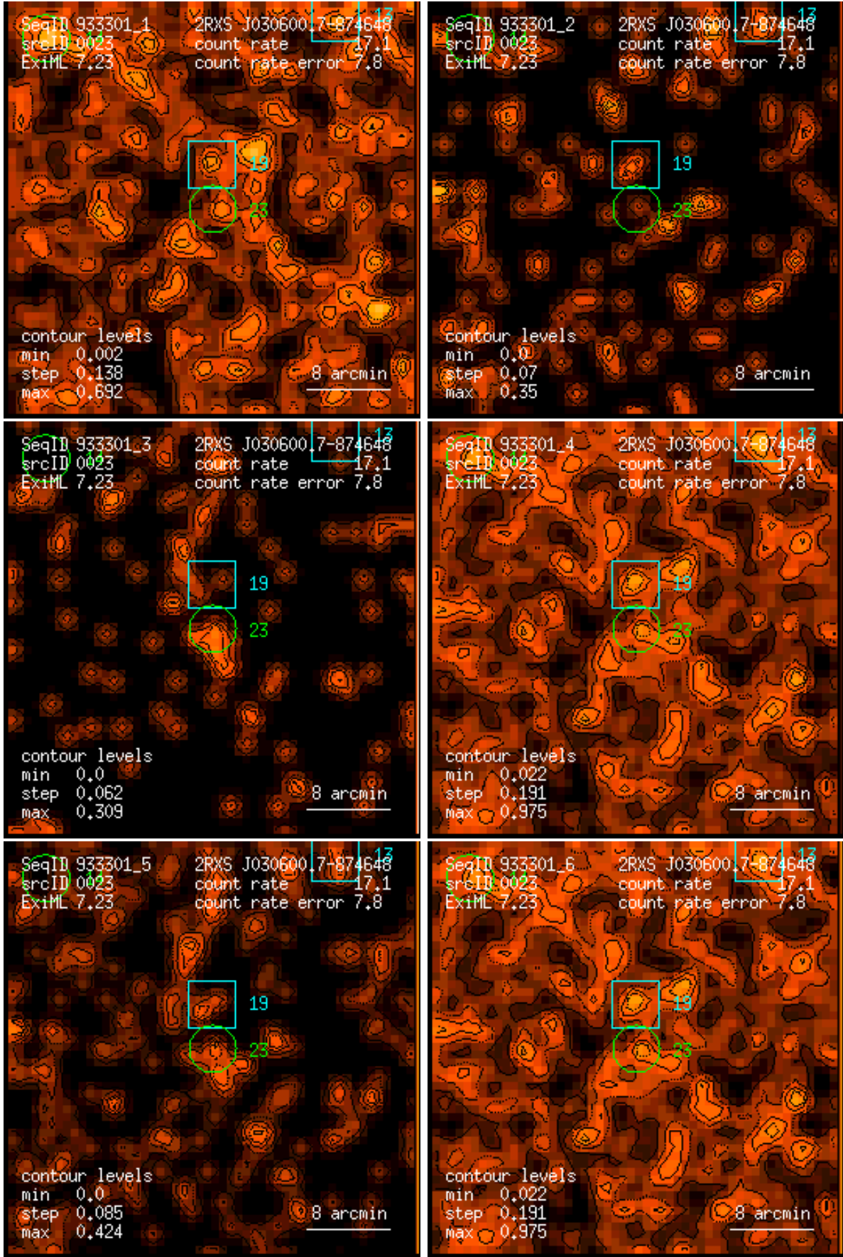
Figure 23: RASS 933301: detection 0023: band rate images, Gaussian filter: (1) PSPC channels 11 – 41, (2) 52 – 90, (3) 91 – 201, (4) 11 – 235, (5) 52 – 201, (6) 11 – 201. Broad band rates in counts/ks. Band rate contour levels in counts/ks/arcmin 2 .
