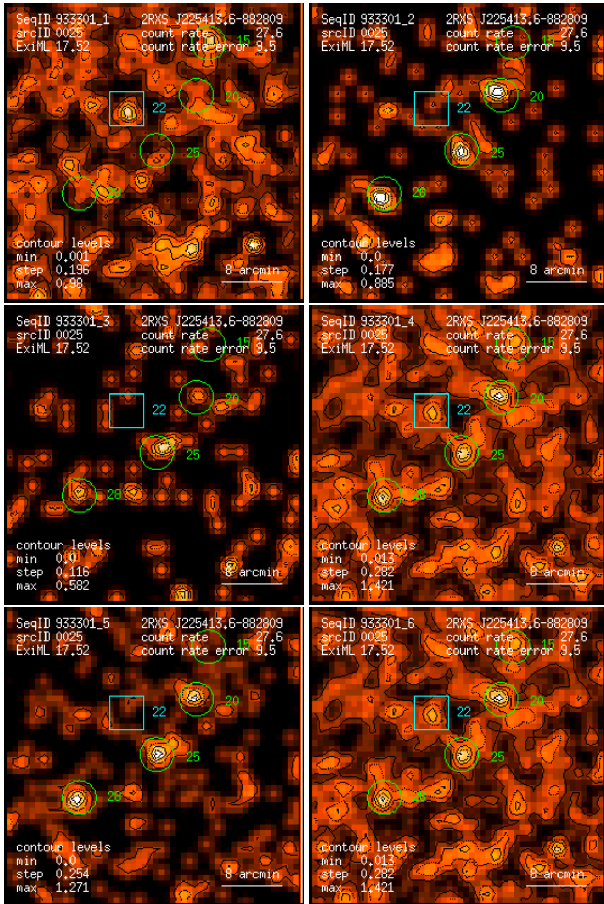
Figure 25: RASS 933301: detection 0025: band rate images, Gaussian filter: (1) PSPC channels 11 – 41, (2) 52 – 90, (3) 91 – 201, (4) 11 – 235, (5) 52 – 201, (6) 11 – 201. Broad band rates in counts/ks. Band rate contour levels in counts/ks/arcmin 2 .
