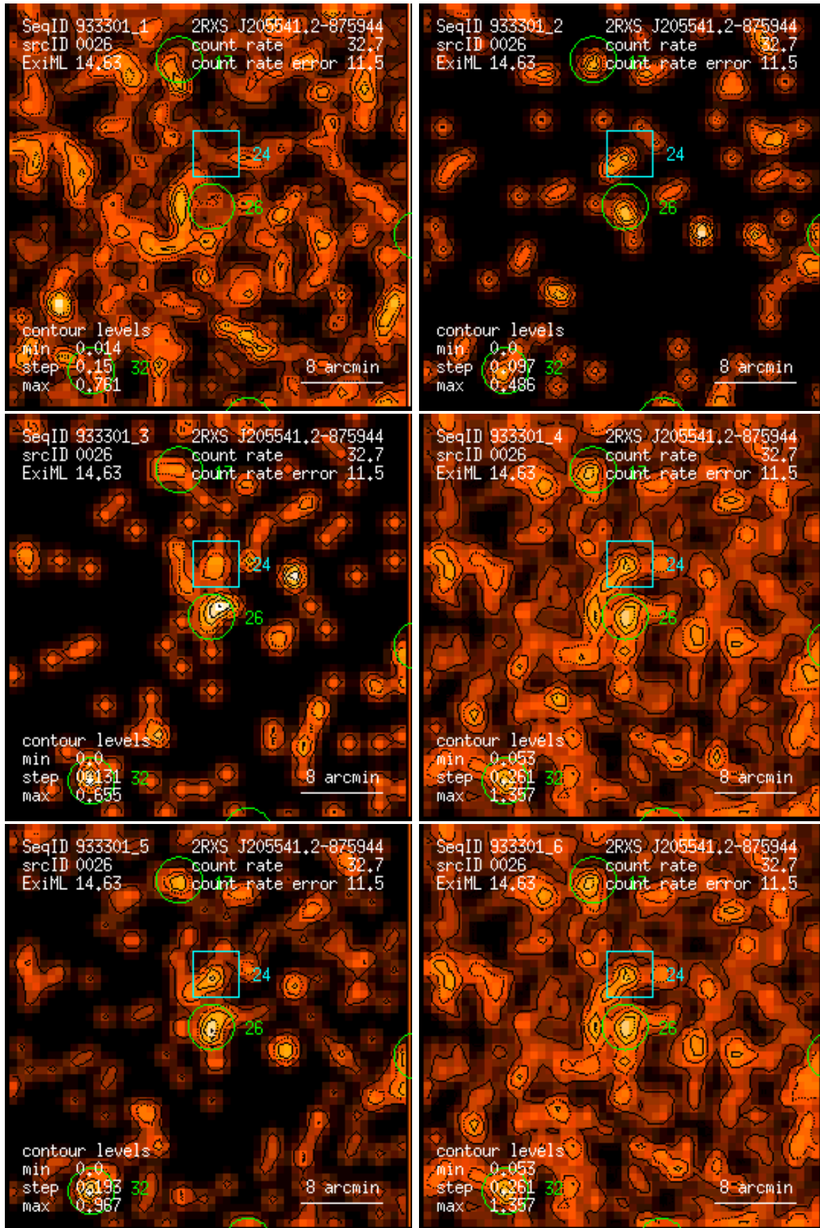
Figure 26: RASS 933301: detection 0026: band rate images, Gaussian filter: (1) PSPC channels 11 – 41, (2) 52 – 90, (3) 91 – 201, (4) 11 – 235, (5) 52 – 201, (6) 11 – 201. Broad band rates in counts/ks. Band rate contour levels in counts/ks/arcmin 2 .
