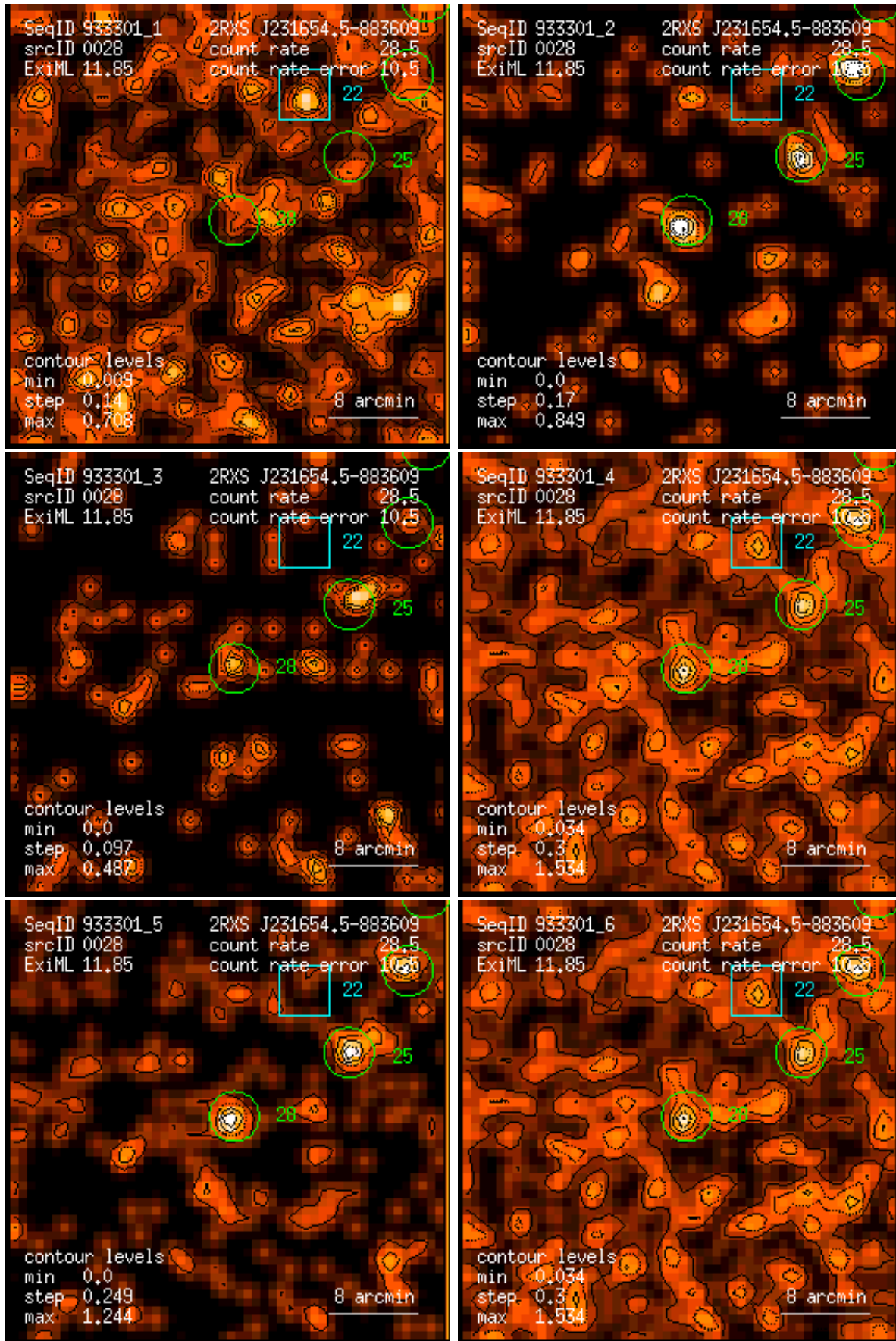
Figure 28: RASS 933301: detection 0028: band rate images, Gaussian filter: (1) PSPC channels 11 – 41, (2) 52 – 90, (3) 91 – 201, (4) 11 – 235, (5) 52 – 201, (6) 11 – 201. Broad band rates in counts/ks. Band rate contour levels in counts/ks/arcmin 2 .
