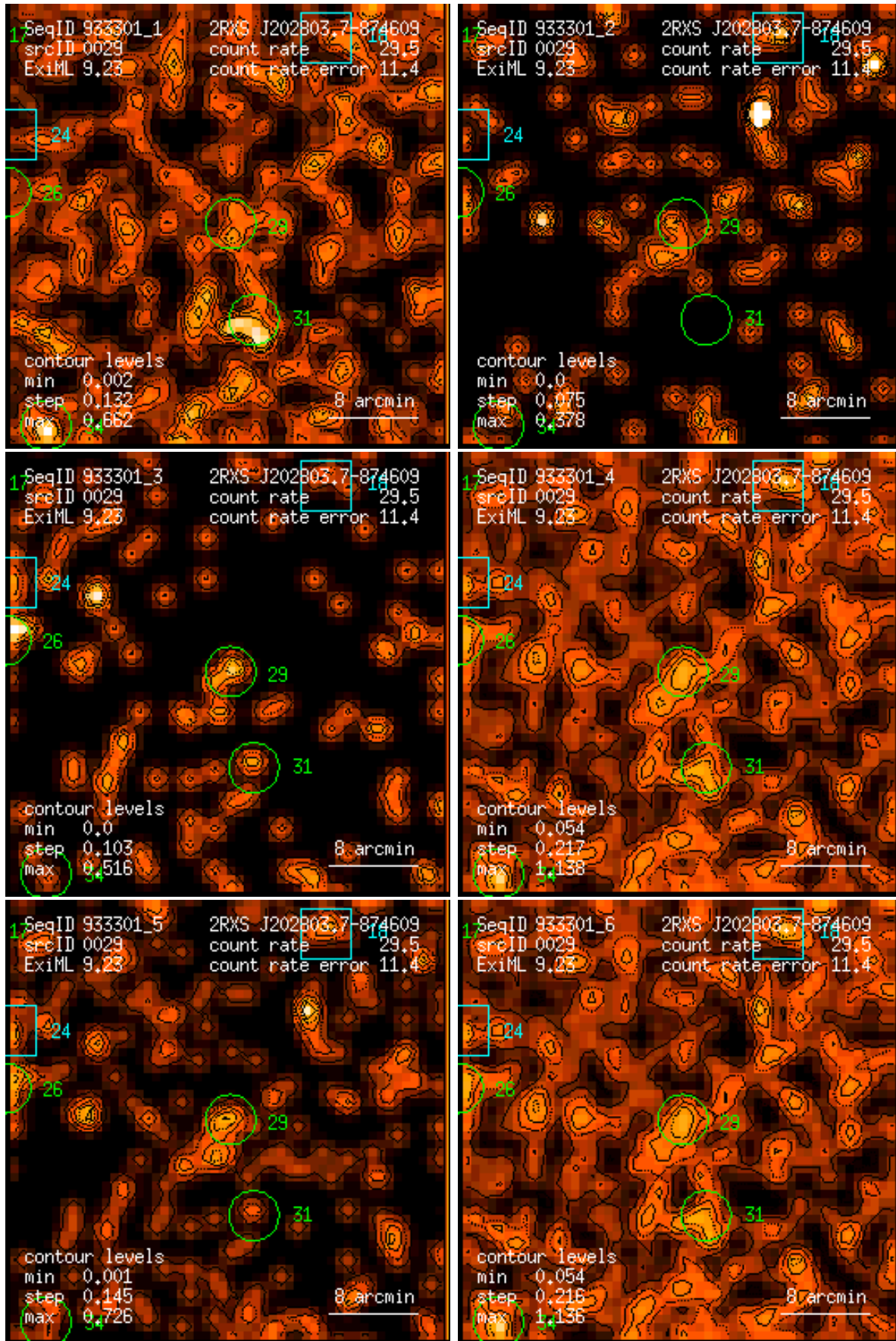
Figure 29: RASS 933301: detection 0029: band rate images, Gaussian filter: (1) PSPC channels 11 – 41, (2) 52 – 90, (3) 91 – 201, (4) 11 – 235, (5) 52 – 201, (6) 11 – 201. Broad band rates in counts/ks. Band rate contour levels in counts/ks/arcmin 2 .
