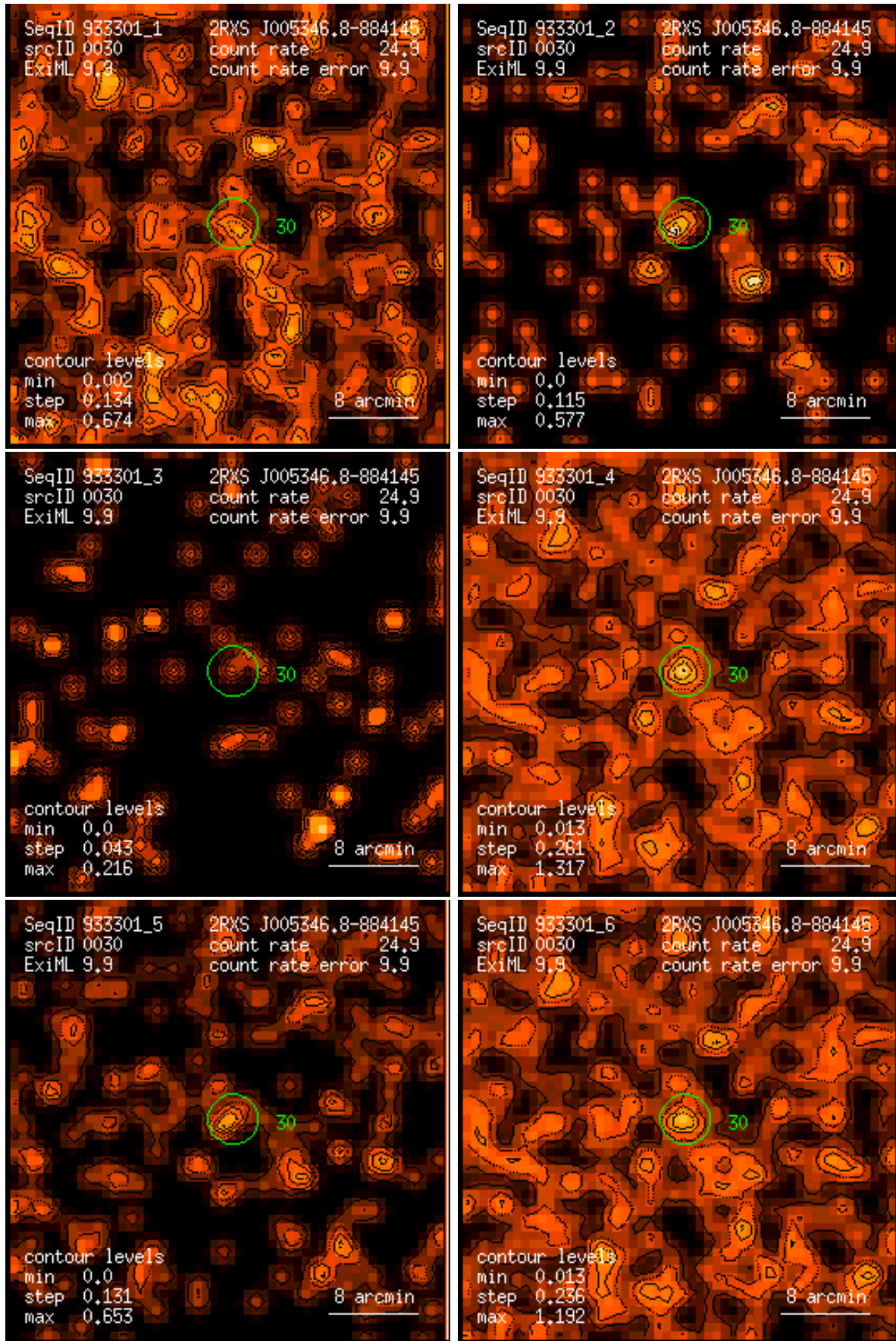
Figure 30: RASS 933301: detection 0030: band rate images, Gaussian filter: (1) PSPC channels 11 – 41, (2) 52 – 90, (3) 91 – 201, (4) 11 – 235, (5) 52 – 201, (6) 11 – 201. Broad band rates in counts/ks. Band rate contour levels in counts/ks/arcmin 2 .
