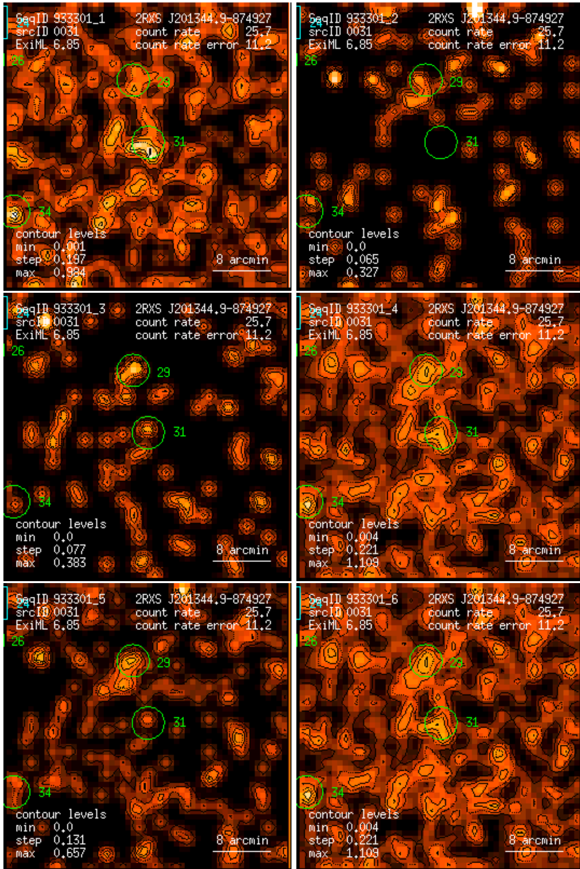
Figure 31: RASS 933301: detection 0031: band rate images, Gaussian filter: (1) PSPC channels 11 – 41, (2) 52 – 90, (3) 91 – 201, (4) 11 – 235, (5) 52 – 201, (6) 11 – 201. Broad band rates in counts/ks. Band rate contour levels in counts/ks/arcmin 2 .
