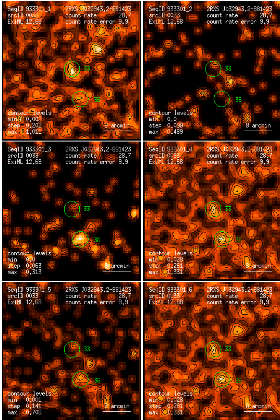
Figure 33: RASS 933301: detection 0033: band rate images, Gaussian filter: (1) PSPC channels 11 – 41, (2) 52 – 90, (3) 91 – 201, (4) 11 – 235, (5) 52 – 201, (6) 11 – 201. Broad band rates in counts/ks. Band rate contour levels in counts/ks/arcmin 2 .
