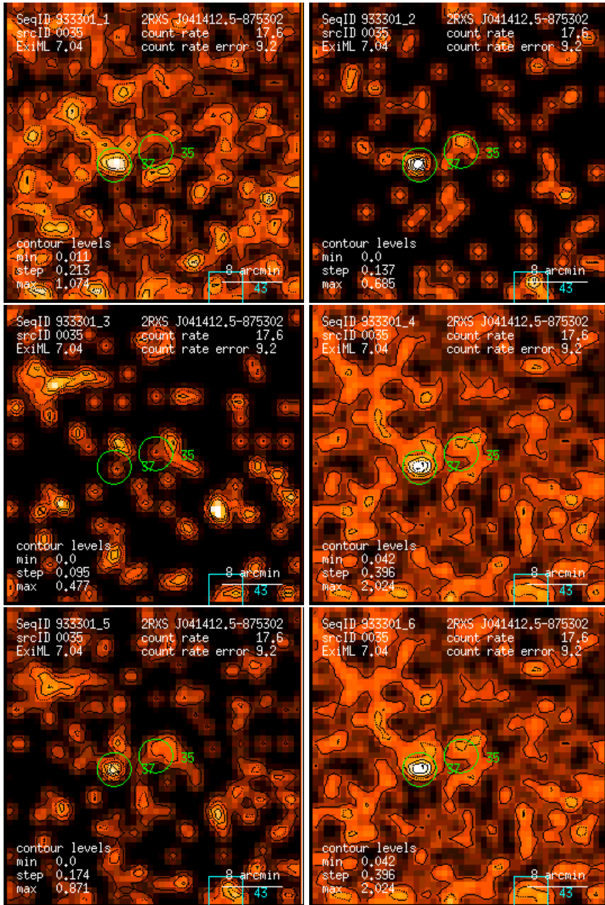
Figure 35: RASS 933301: detection 0035: band rate images, Gaussian filter: (1) PSPC channels 11 – 41, (2) 52 – 90, (3) 91 – 201, (4) 11 – 235, (5) 52 – 201, (6) 11 – 201. Broad band rates in counts/ks. Band rate contour levels in counts/ks/arcmin 2 .
