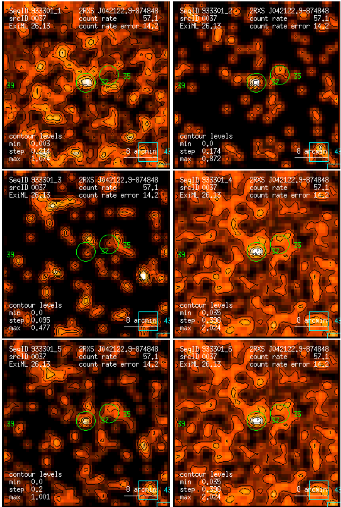
Figure 37: RASS 933301: detection 0037: band rate images, Gaussian filter: (1) PSPC channels 11 – 41, (2) 52 – 90, (3) 91 – 201, (4) 11 – 235, (5) 52 – 201, (6) 11 – 201. Broad band rates in counts/ks. Band rate contour levels in counts/ks/arcmin 2 .
