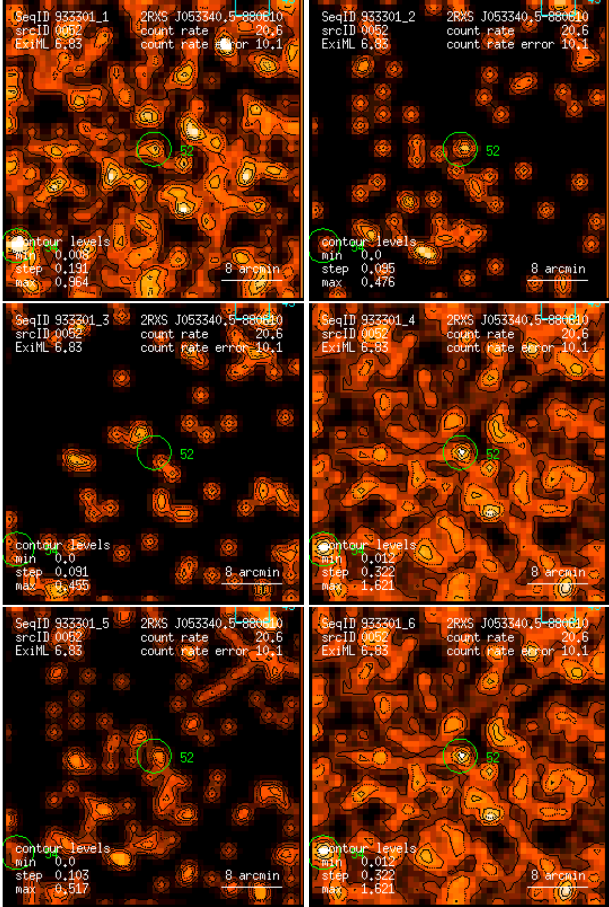
Figure 52: RASS 933301: detection 0052: band rate images, Gaussian filter: (1) PSPC channels 11 – 41, (2) 52 – 90, (3) 91 – 201, (4) 11 – 235, (5) 52 – 201, (6) 11 – 201. Broad band rates in counts/ks. Band rate contour levels in counts/ks/arcmin 2 .
