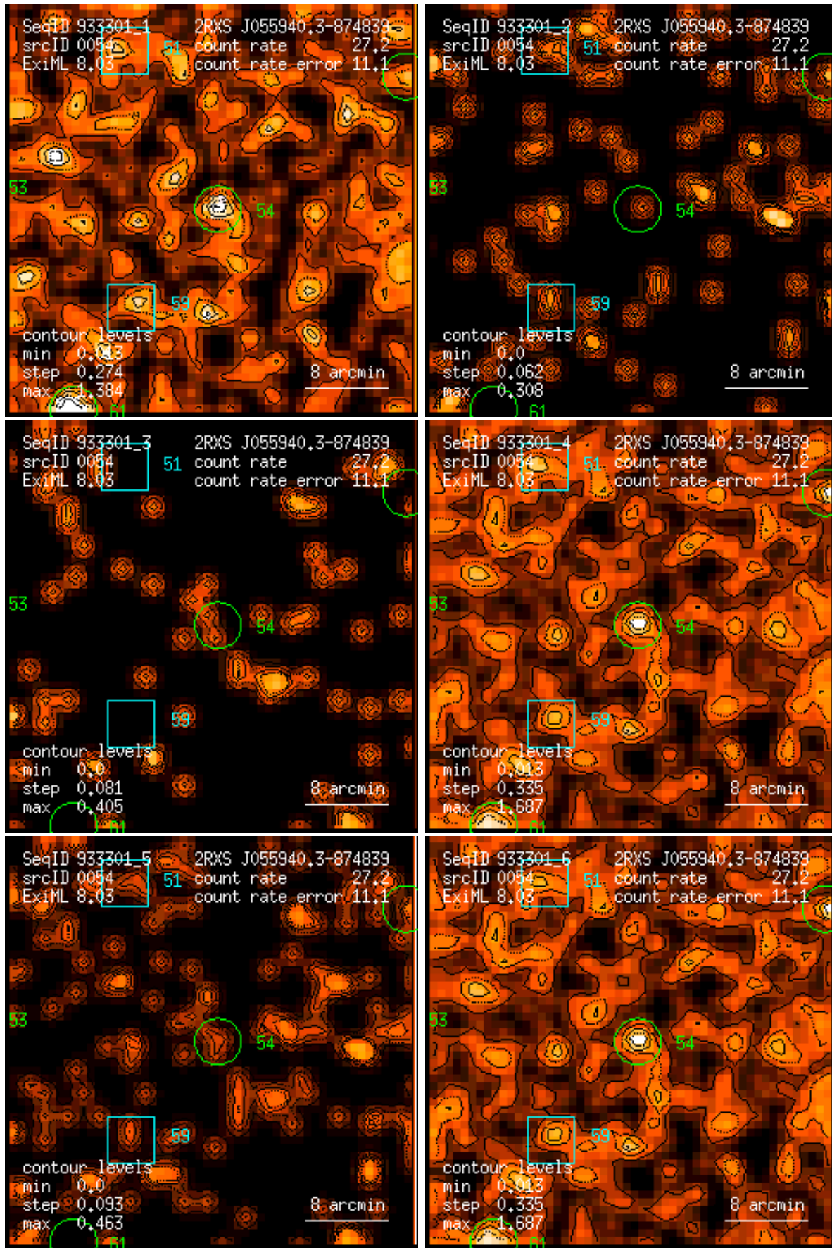
Figure 54: RASS 933301: detection 0054: band rate images, Gaussian filter: (1) PSPC channels 11 – 41, (2) 52 – 90, (3) 91 – 201, (4) 11 – 235, (5) 52 – 201, (6) 11 – 201. Broad band rates in counts/ks. Band rate contour levels in counts/ks/arcmin 2 .
