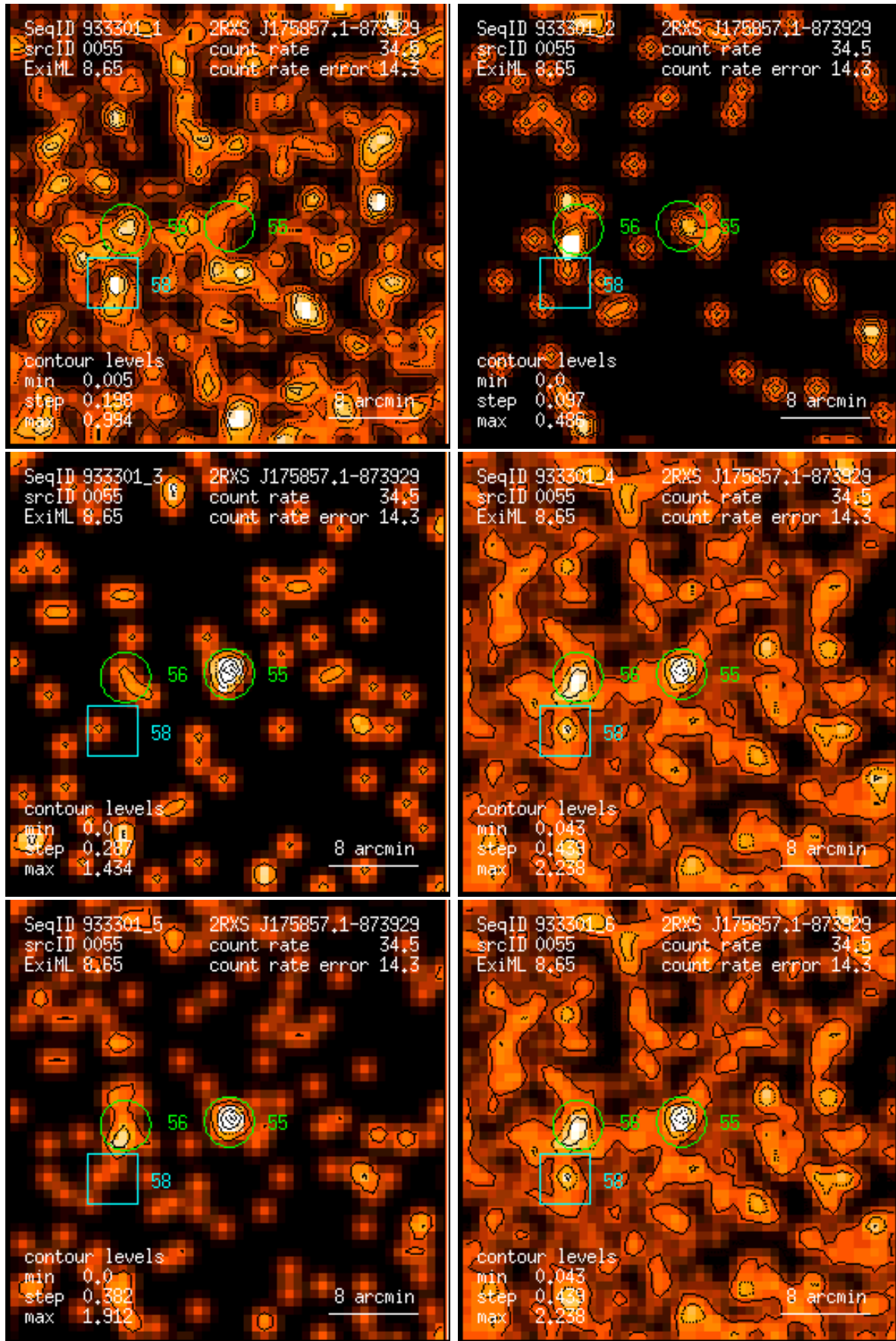
Figure 55: RASS 933301: detection 0055: band rate images, Gaussian filter: (1) PSPC channels 11 – 41, (2) 52 – 90, (3) 91 – 201, (4) 11 – 235, (5) 52 – 201, (6) 11 – 201. Broad band rates in counts/ks. Band rate contour levels in counts/ks/arcmin 2 .
