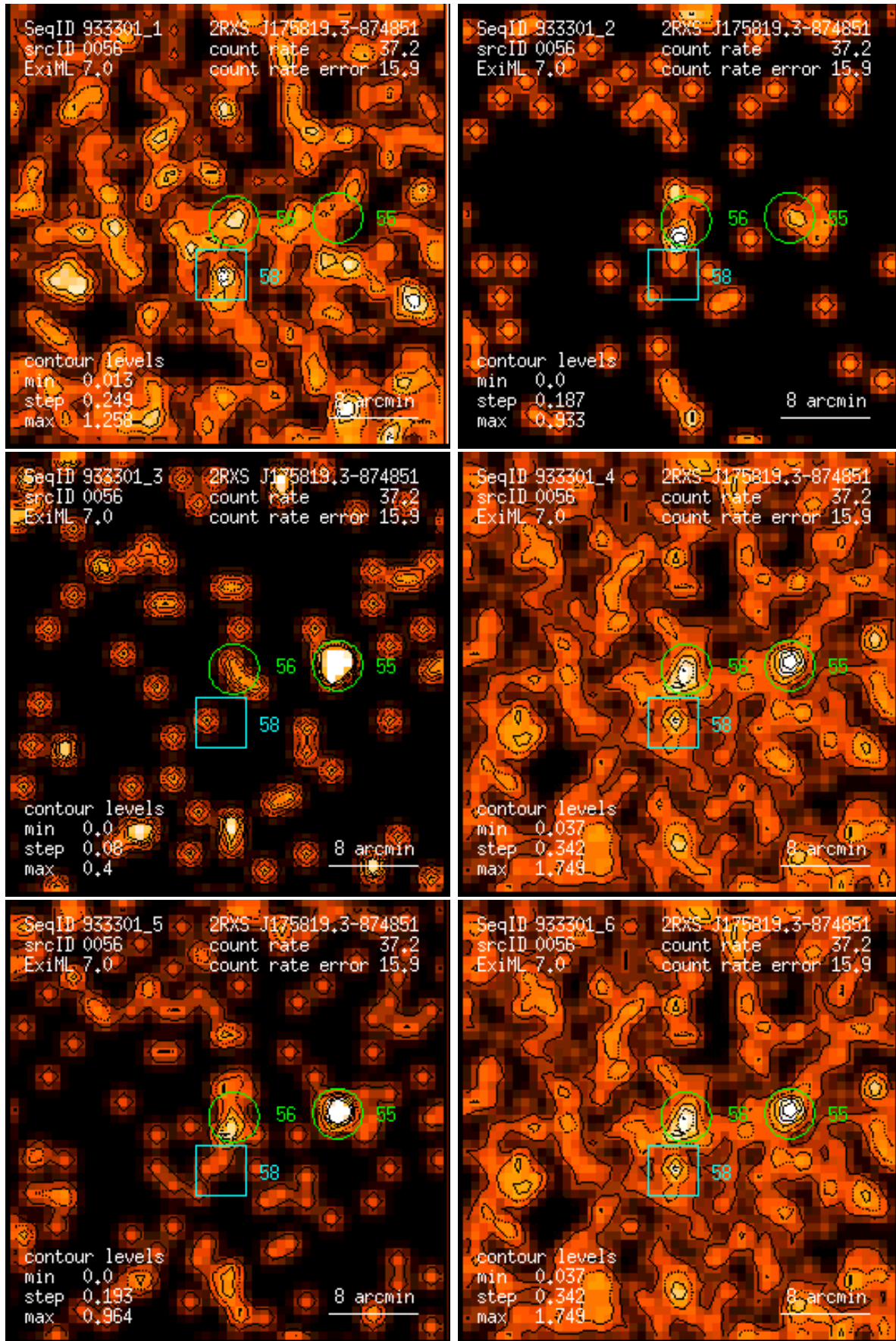
Figure 56: RASS 933301: detection 0056: band rate images, Gaussian filter: (1) PSPC channels 11 – 41, (2) 52 – 90, (3) 91 – 201, (4) 11 – 235, (5) 52 – 201, (6) 11 – 201. Broad band rates in counts/ks. Band rate contour levels in counts/ks/arcmin 2 .
