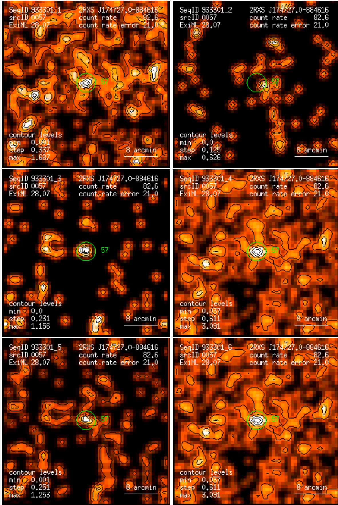
Figure 57: RASS 933301: detection 0057: band rate images, Gaussian filter: (1) PSPC channels 11 – 41, (2) 52 – 90, (3) 91 – 201, (4) 11 – 235, (5) 52 – 201, (6) 11 – 201. Broad band rates in counts/ks. Band rate contour levels in counts/ks/arcmin 2 .
