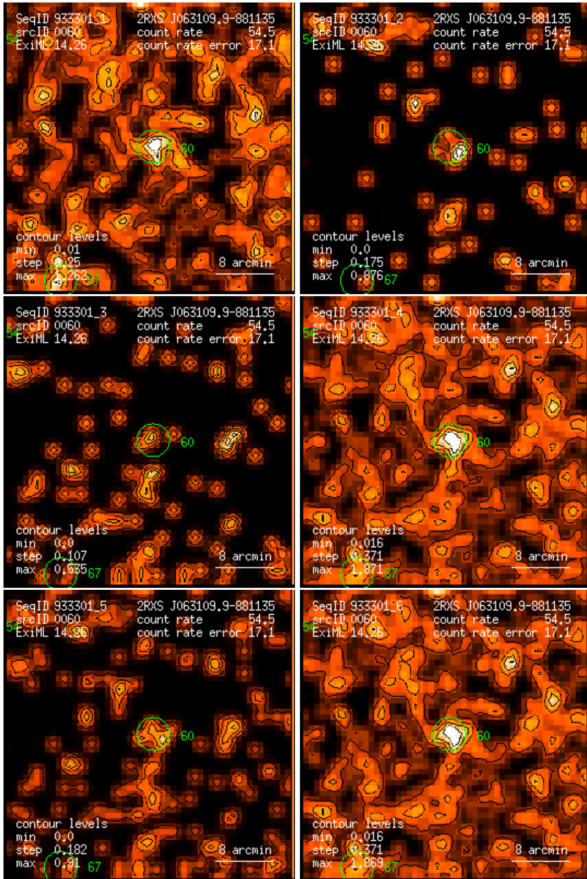
Figure 60: RASS 933301: detection 0060: band rate images, Gaussian filter: (1) PSPC channels 11 – 41, (2) 52 – 90, (3) 91 – 201, (4) 11 – 235, (5) 52 – 201, (6) 11 – 201. Broad band rates in counts/ks. Band rate contour levels in counts/ks/arcmin 2 .
