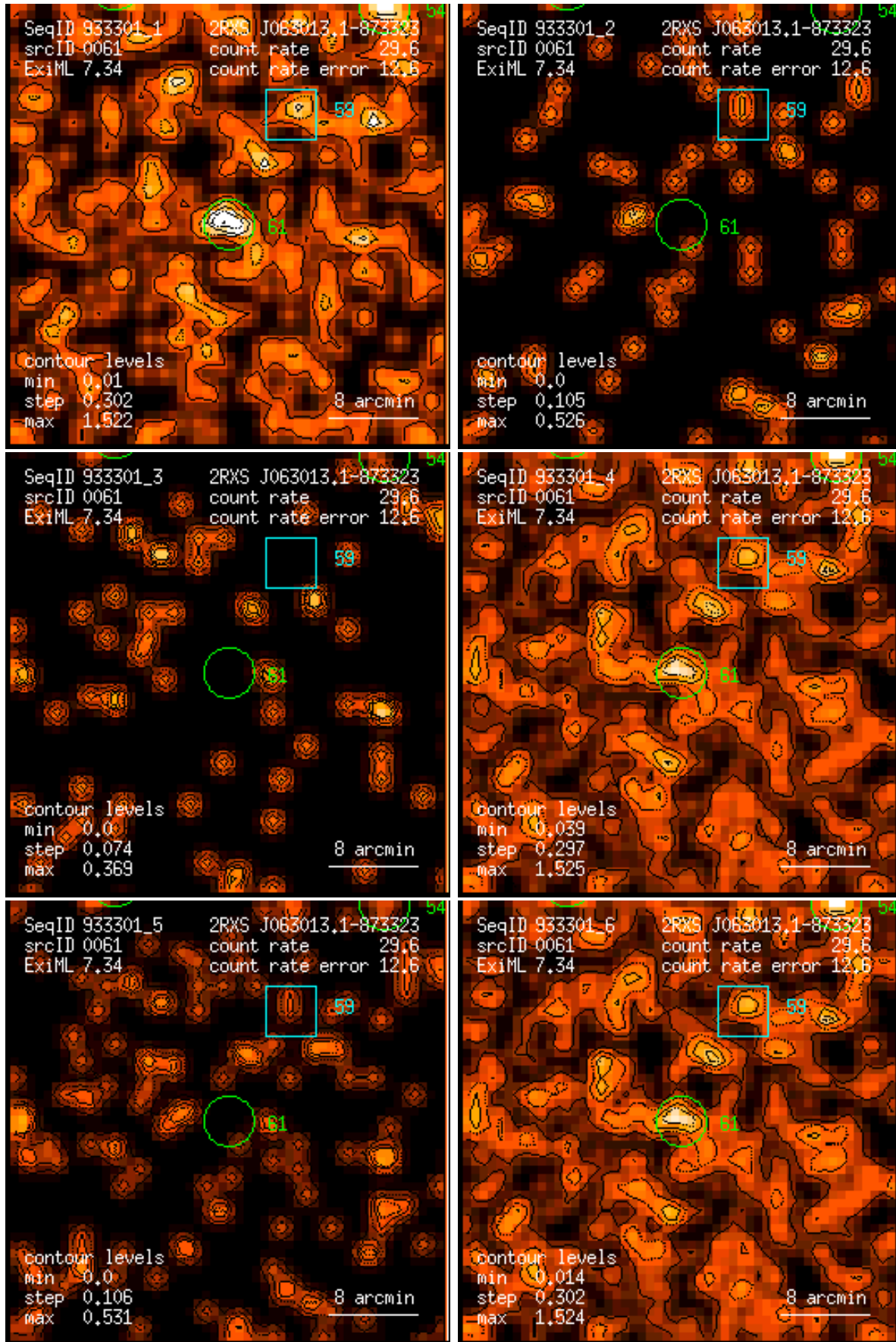
Figure 61: RASS 933301: detection 0061: band rate images, Gaussian filter: (1) PSPC channels 11 – 41, (2) 52 – 90, (3) 91 – 201, (4) 11 – 235, (5) 52 – 201, (6) 11 – 201. Broad band rates in counts/ks. Band rate contour levels in counts/ks/arcmin 2 .
