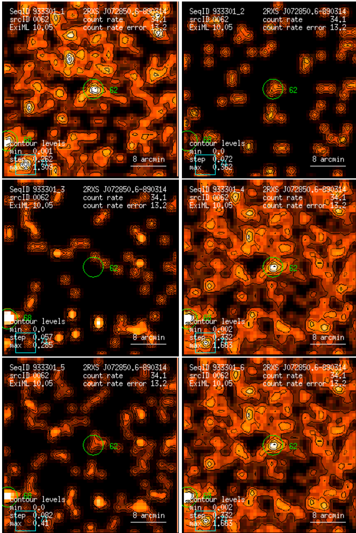
Figure 62: RASS 933301: detection 0062: band rate images, Gaussian filter: (1) PSPC channels 11 – 41, (2) 52 – 90, (3) 91 – 201, (4) 11 – 235, (5) 52 – 201, (6) 11 – 201. Broad band rates in counts/ks. Band rate contour levels in counts/ks/arcmin 2 .
