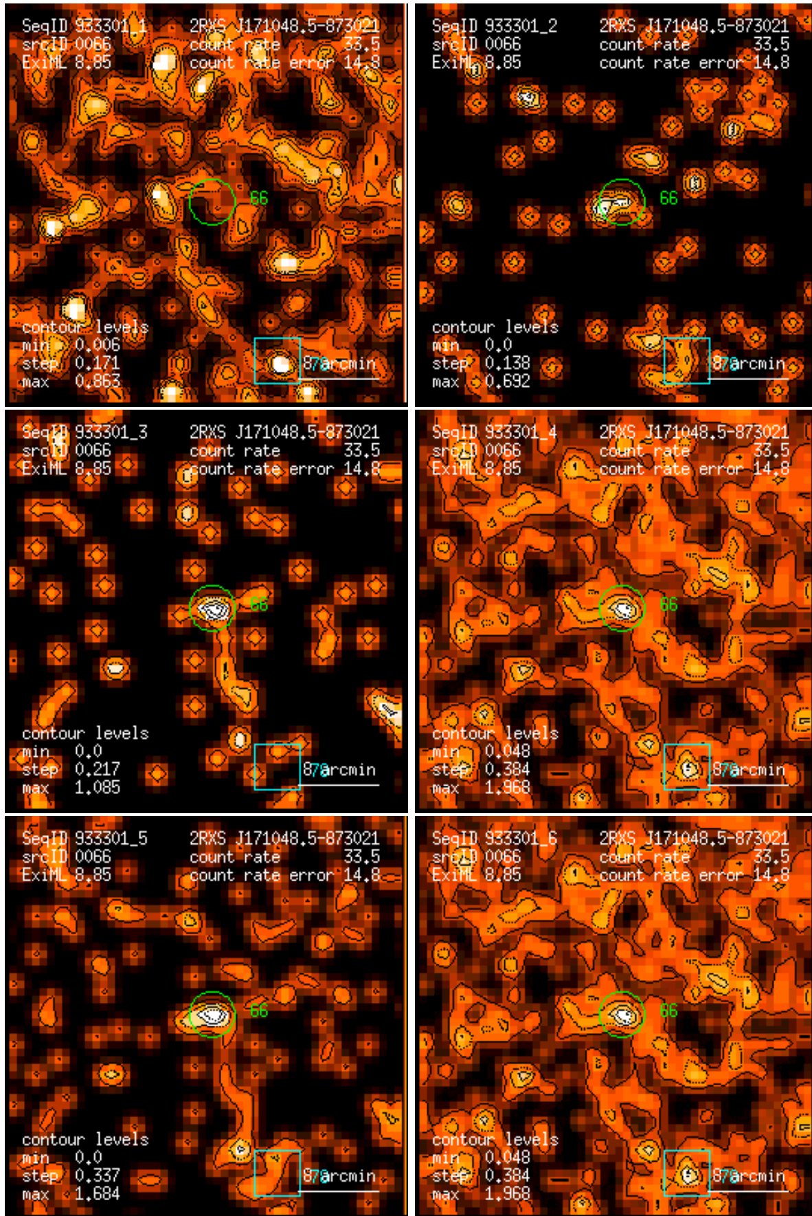
Figure 66: RASS 933301: detection 0066: band rate images, Gaussian filter: (1) PSPC channels 11 – 41, (2) 52 – 90, (3) 91 – 201, (4) 11 – 235, (5) 52 – 201, (6) 11 – 201. Broad band rates in counts/ks. Band rate contour levels in counts/ks/arcmin 2 .
