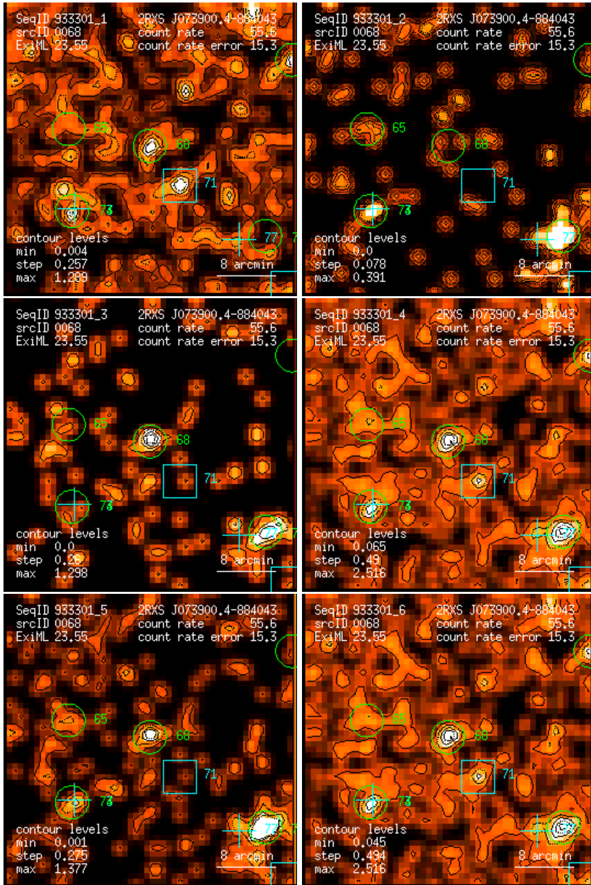
Figure 68: RASS 933301: detection 0068: band rate images, Gaussian filter: (1) PSPC channels 11 – 41, (2) 52 – 90, (3) 91 – 201, (4) 11 – 235, (5) 52 – 201, (6) 11 – 201. Broad band rates in counts/ks. Band rate contour levels in counts/ks/arcmin 2 .
