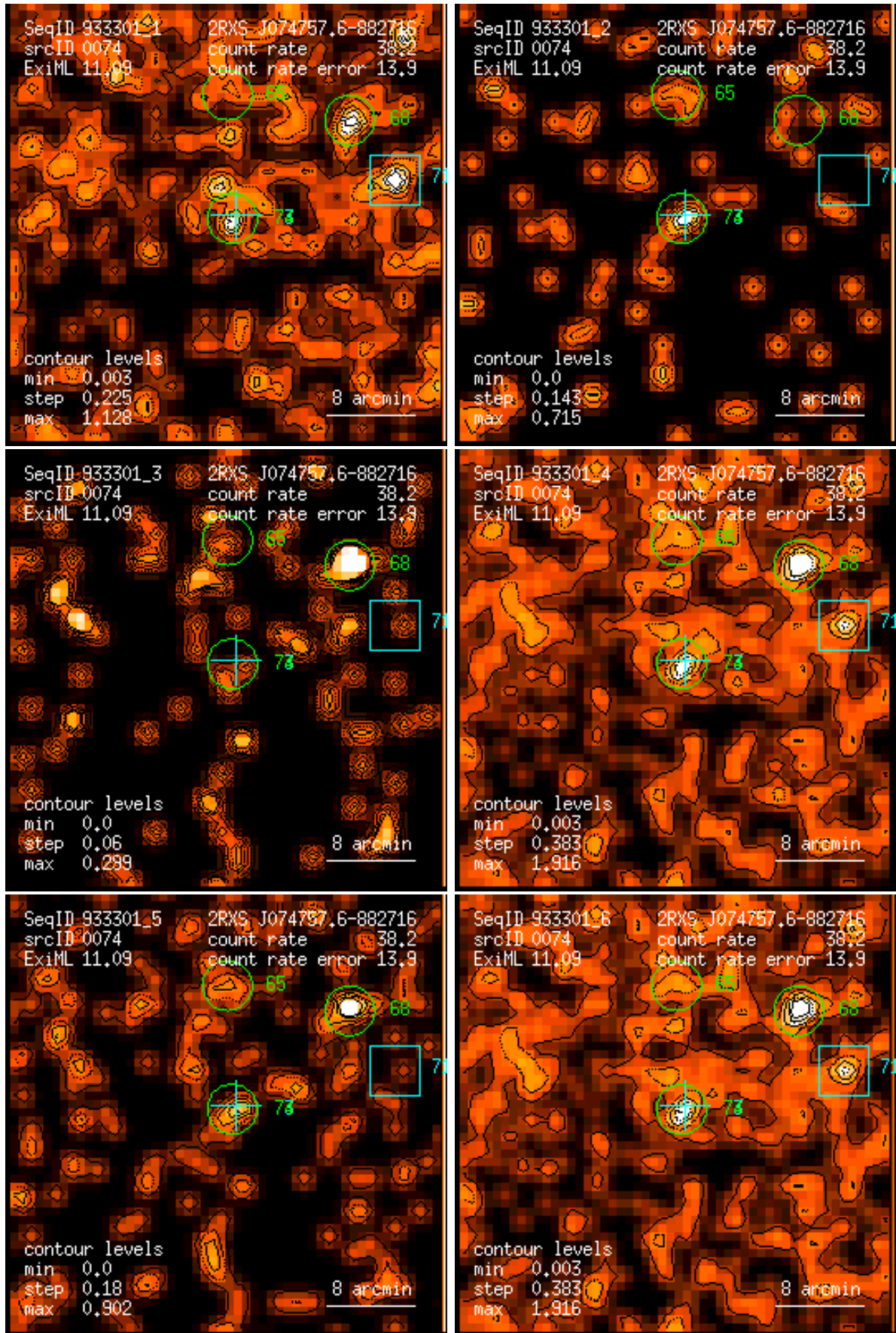
Figure 74: RASS 933301: detection 0074: band rate images, Gaussian filter: (1) PSPC channels 11 – 41, (2) 52 – 90, (3) 91 – 201, (4) 11 – 235, (5) 52 – 201, (6) 11 – 201. Broad band rates in counts/ks. Band rate contour levels in counts/ks/arcmin 2 .
