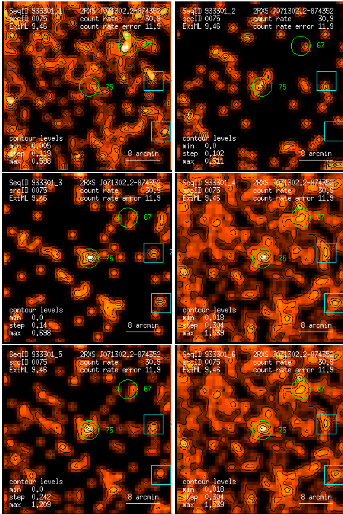
Figure 75: RASS 933301: detection 0075: band rate images, Gaussian filter: (1) PSPC channels 11 – 41, (2) 52 – 90, (3) 91 – 201, (4) 11 – 235, (5) 52 – 201, (6) 11 – 201. Broad band rates in counts/ks. Band rate contour levels in counts/ks/arcmin 2 .
