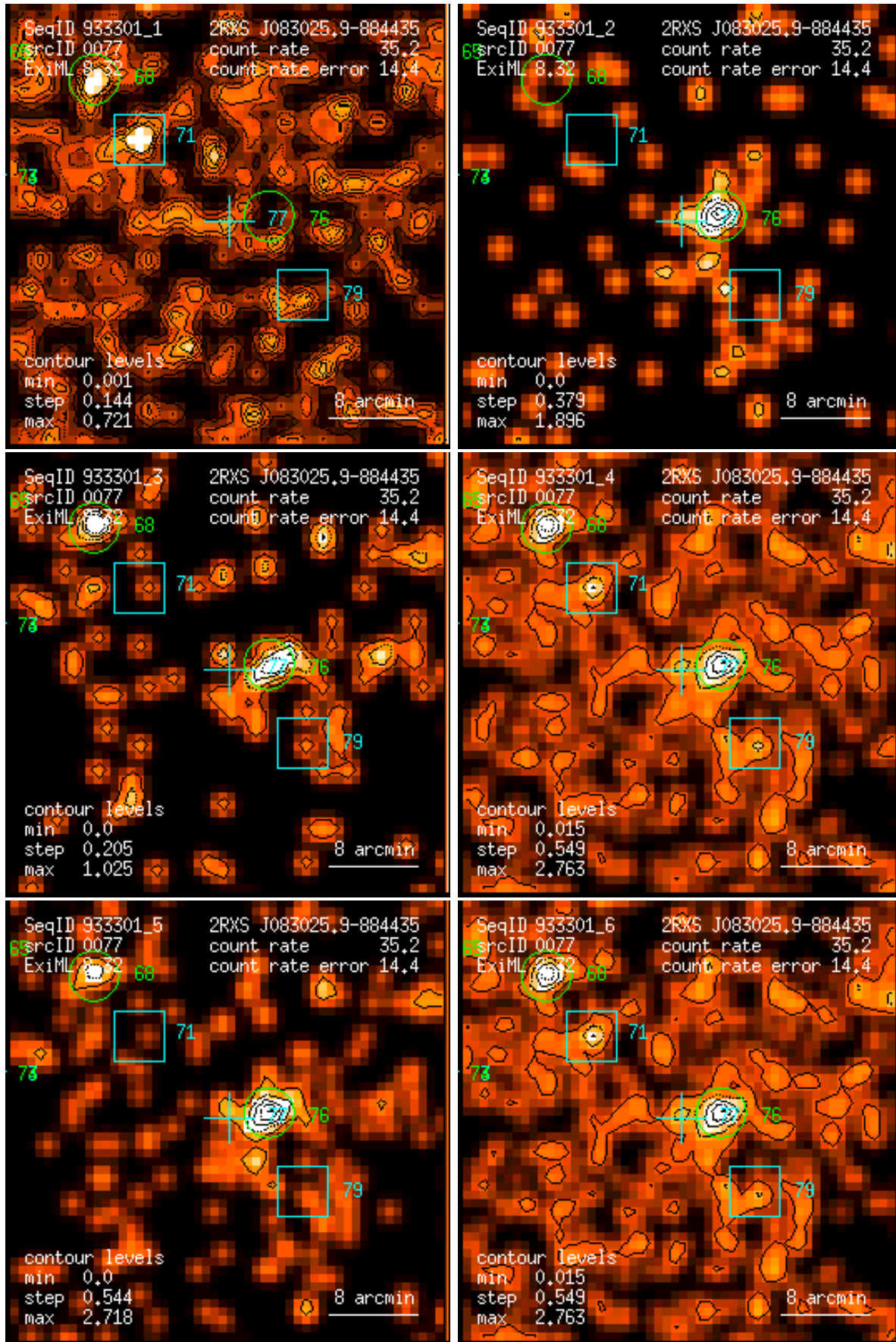
Figure 77: RASS 933301: detection 0077: band rate images, Gaussian filter: (1) PSPC channels 11 – 41, (2) 52 – 90, (3) 91 – 201, (4) 11 – 235, (5) 52 – 201, (6) 11 – 201. Broad band rates in counts/ks. Band rate contour levels in counts/ks/arcmin 2 .
