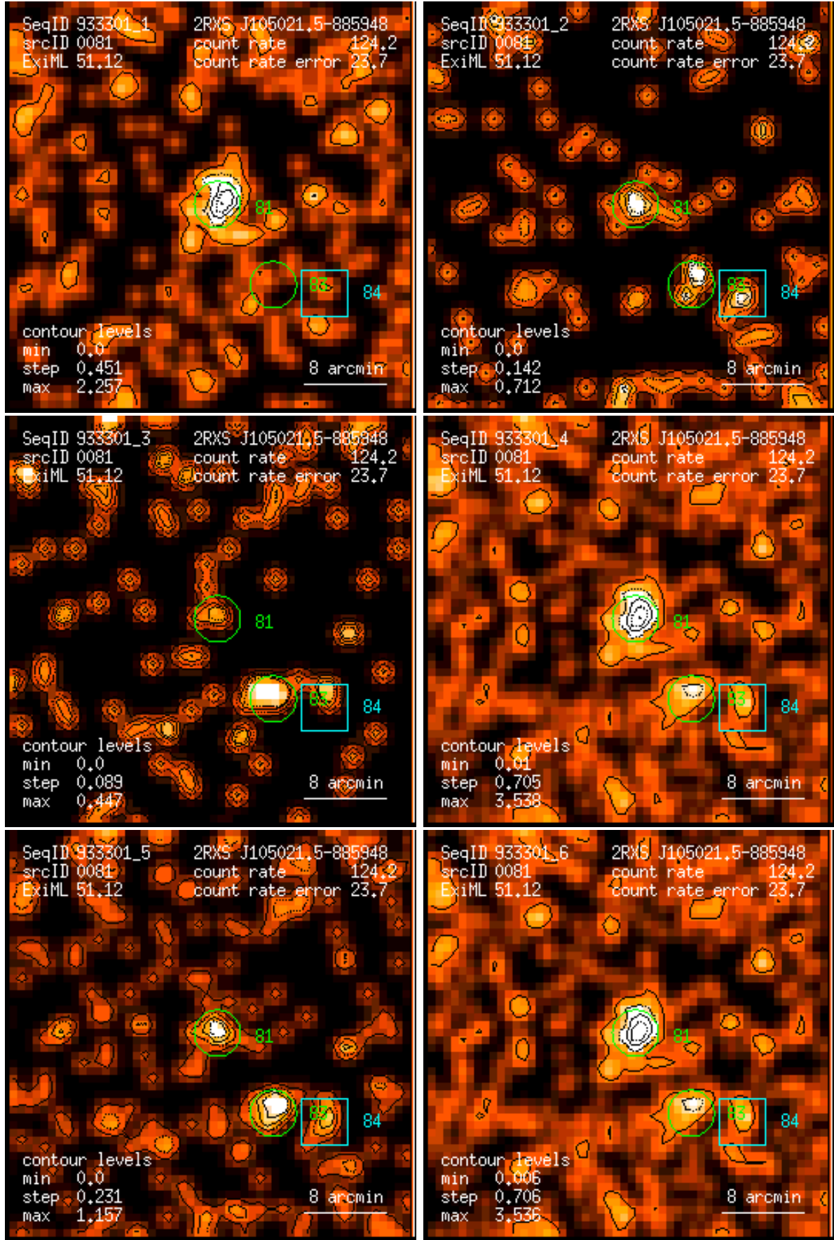
Figure 81: RASS 933301: detection 0081: band rate images, Gaussian filter: (1) PSPC channels 11 – 41, (2) 52 – 90, (3) 91 – 201, (4) 11 – 235, (5) 52 – 201, (6) 11 – 201. Broad band rates in counts/ks. Band rate contour levels in counts/ks/arcmin 2 .
