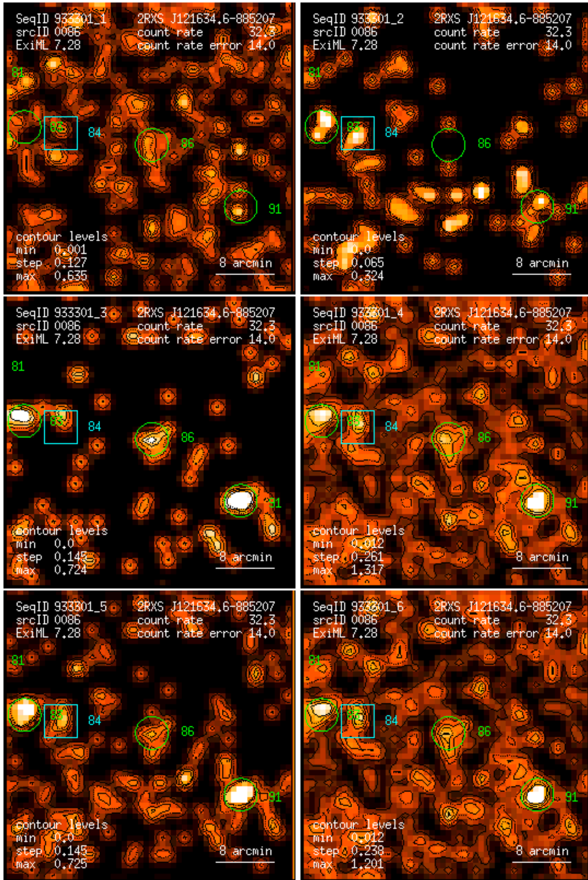
Figure 86: RASS 933301: detection 0086: band rate images, Gaussian filter: (1) PSPC channels 11 – 41, (2) 52 – 90, (3) 91 – 201, (4) 11 – 235, (5) 52 – 201, (6) 11 – 201. Broad band rates in counts/ks. Band rate contour levels in counts/ks/arcmin 2 .
