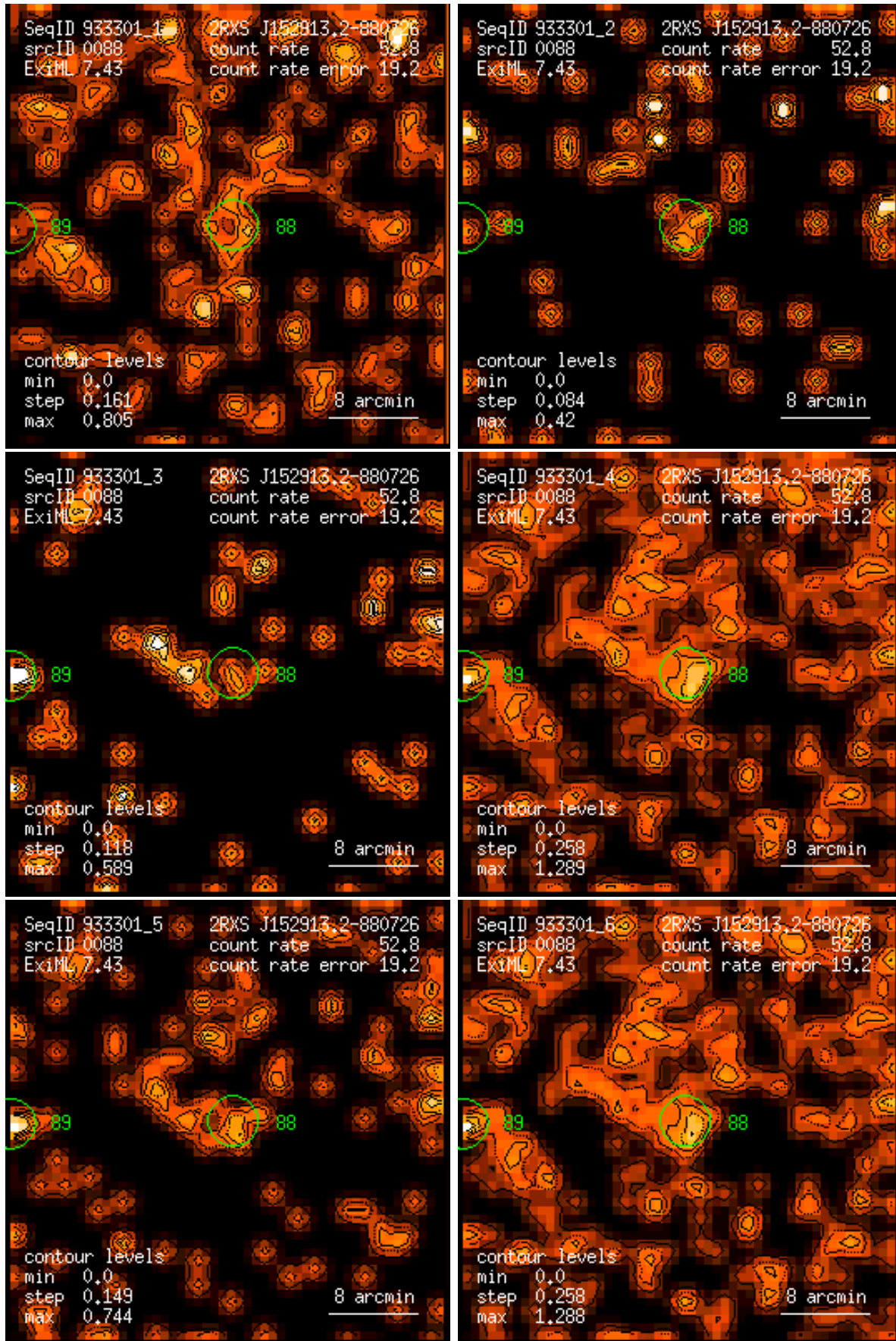
Figure 88: RASS 933301: detection 0088: band rate images, Gaussian filter: (1) PSPC channels 11 – 41, (2) 52 – 90, (3) 91 – 201, (4) 11 – 235, (5) 52 – 201, (6) 11 – 201. Broad band rates in counts/ks. Band rate contour levels in counts/ks/arcmin 2 .
