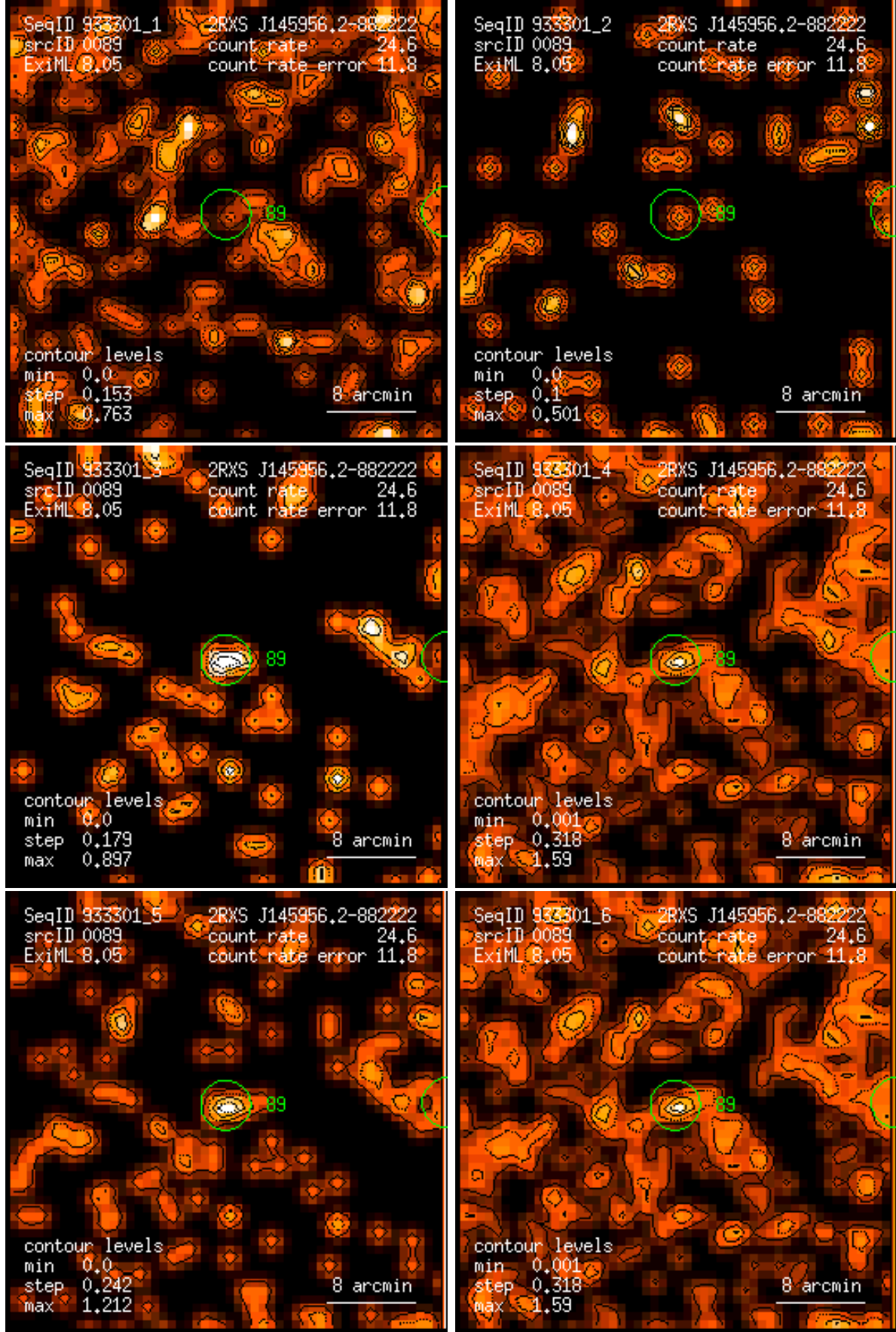
Figure 89: RASS 933301: detection 0089: band rate images, Gaussian filter: (1) PSPC channels 11 – 41, (2) 52 – 90, (3) 91 – 201, (4) 11 – 235, (5) 52 – 201, (6) 11 – 201. Broad band rates in counts/ks. Band rate contour levels in counts/ks/arcmin 2 .
